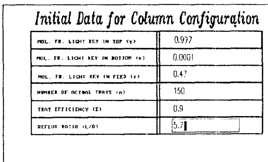
Fig. 17. Distillation column spec.
