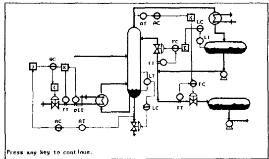
Fig. 20. Regulatory controls.
