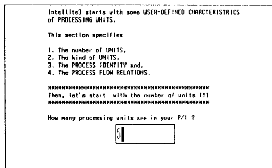
Fig. 13. Inputting the number of units.
