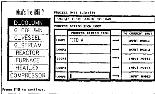
Fig. 14. Unit & stream specification.
