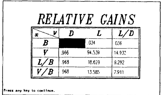
Fig. 18. Computed RGA.
