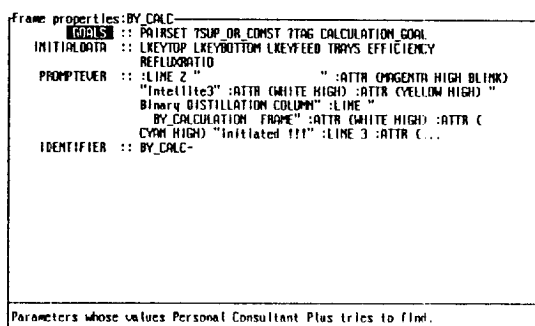
Fig. 9. Task Frame properties of BY_CALC.
