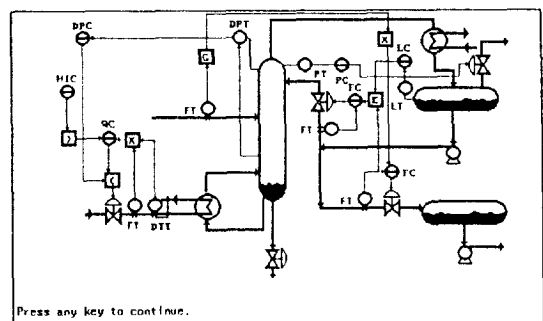
Fig. 21. Constraint & supportive controls.
