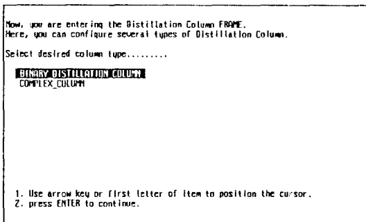
Fig. 15. Selecting distillation column type.
