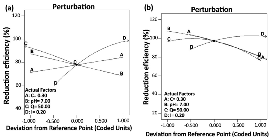
Fig. 4. Perturbation plots for Cr(VI) reduction by (a) Copper foam cathode and (b) PdNPs coated copper foam.
