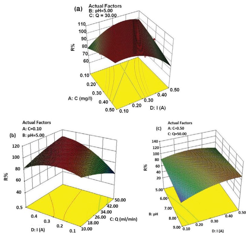
Fig. S1. The 3D response surface plots for the case of using copper foam cathode for interactive effect of (a) current intensity and initial concentration of Cr(VI); pH at 5 and flow rate at 30 mL/min, (b) flow rate and current intensity; pH at 5 and initial concentration at 0.1 mg L -1 , (c) pH and current intensity; flow rate at 50 mLmin -1 (maximum level) and initial concentration at 0.5 mg L -1 .
