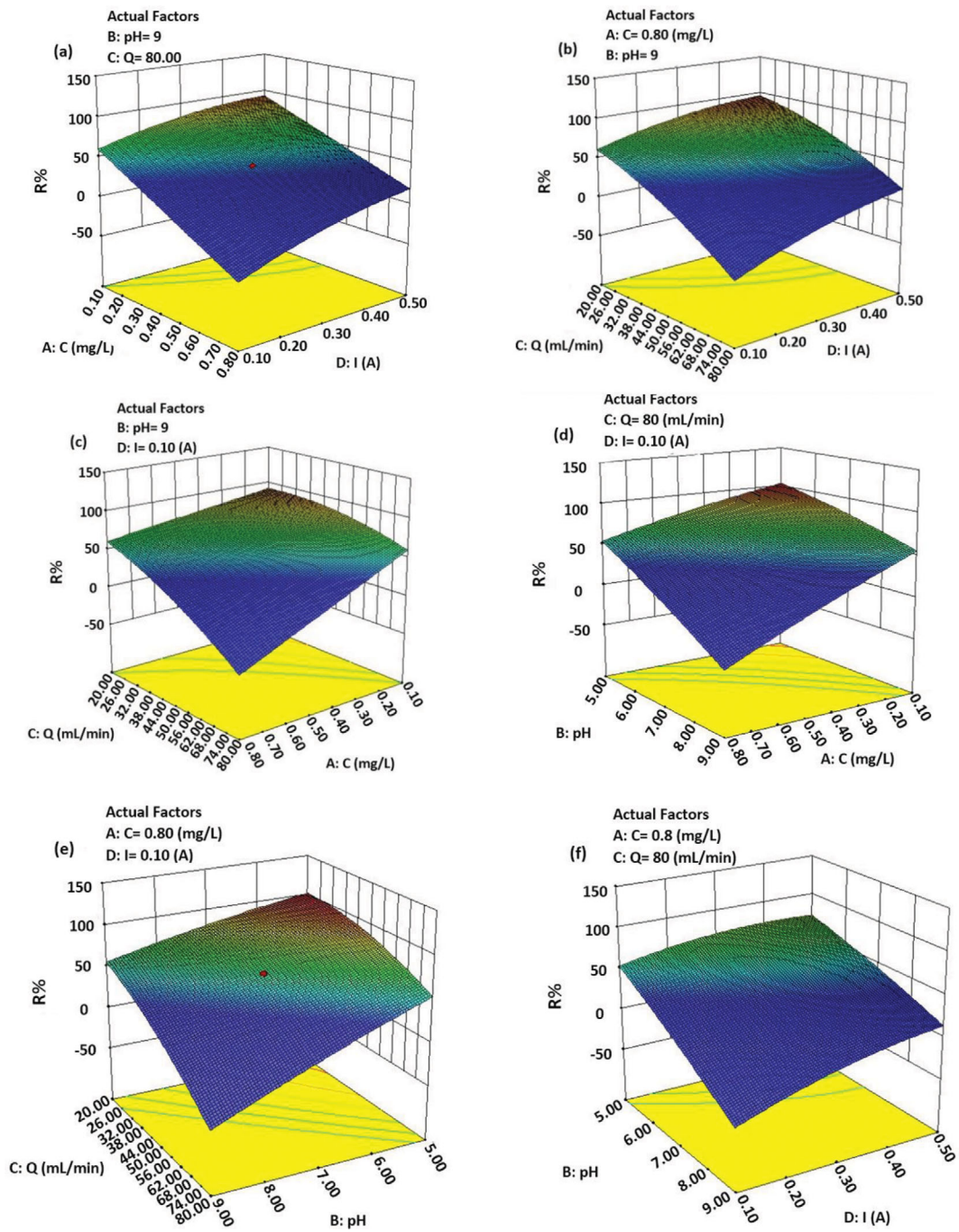
Fig. S2. The 3D response surface plots for the case of using copper foam cathode coated with PdNPs for interactive effect of (a) current intensity and initial concentration of Cr(VI), (b) flow rate and current intensity, (c) flow rate and initial concentration, (d) pH value and initial concentration, (e) pH value and flow rate, (f) pH value and current intensity.
