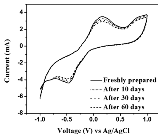
Fig. S2. Stability test of freshly prepared CuO@Ac/Cp electrode and after 10, 30 and 60 days.
