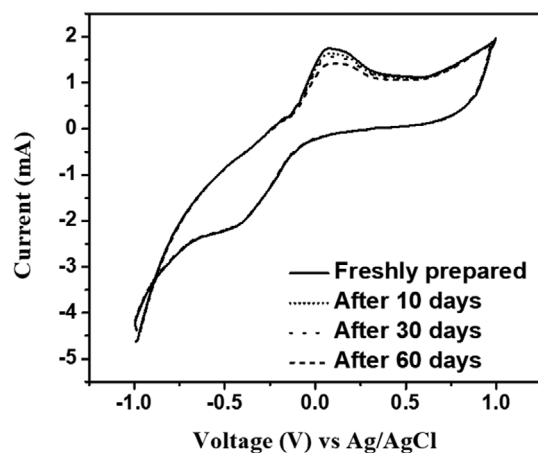
Fig. S1. Stability test of freshly prepared Cu@Ac/Cp electrode and after 10, 30 and 60 days.
