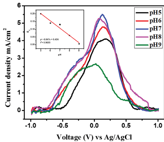
Fig. S3. Cyclic voltammety and effect of peak potential of CuO@Ac/Cp in 0.1 M PBS with 2 mM AMX at various pH values.
