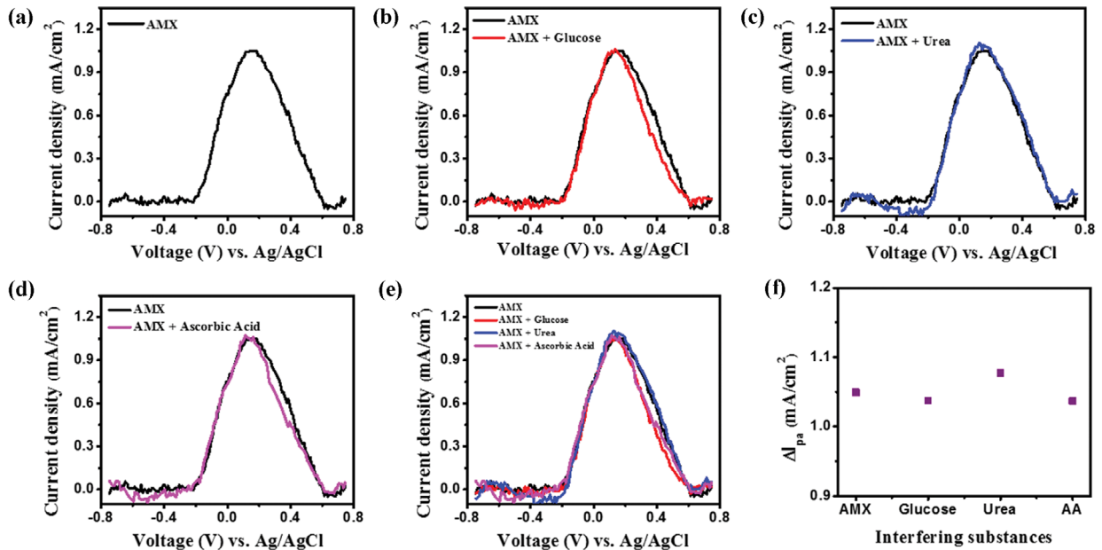
Fig. S4. Interference studies of various substances for the detection of AMX (200 \mu M) in 0.1 M PBS (pH 7).
