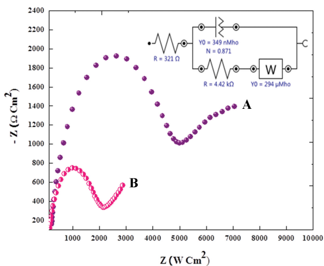
Fig. 3. The Nyquist plot of the (A) CPE and (B) MWCNTs/CPE in phosphate buffer in the presence of 5.0 \text{ mM } [\text{Fe}(\text{CN})_6]^{3-/4-} .
