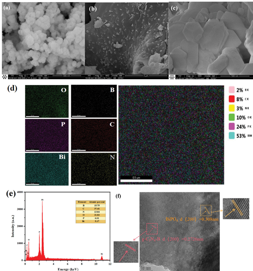
Fig. 2. SEM images of \text{BiPO}_4 (a), \text{g-C}_3\text{N}_4\text{-B} (b), and 1:2BP-CB (c); element map (d), EDS map (e), and HR-TEM map (f) of 1:2BP-CB.
