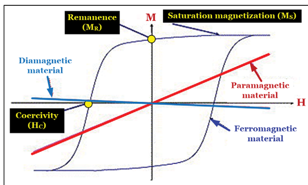
Fig. S4. A magnetisation vs. field strength for a ferromagnetic and a paramagnetic material (adapted from Waters et al. [3]).
