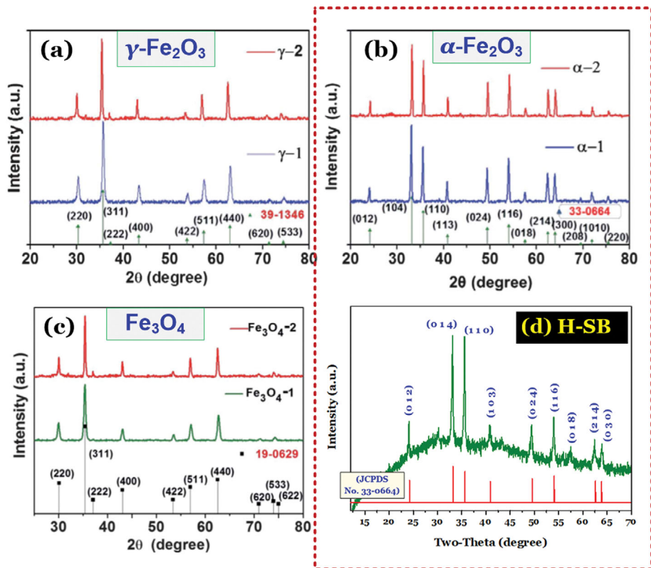
Fig. S2. Comparison of the XRD spectrum of iron oxides nanoparticles: (a) maghemite \gamma\text{-Fe}_2\text{O}_3 , (b) hematite \alpha\text{-Fe}_2\text{O}_3 , and (c) magnetite \text{Fe}_3\text{O}_4 (adapted from Dar and Shivashankar [2]) and (d) that of H-SB in this study. The result of comparison confirmed that the dominant form of the oxides nanoparticles in the surface of H-SB was \alpha\text{-Fe}_2\text{O}_3 .
