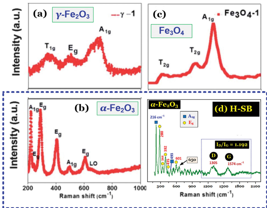
Fig. S3. Comparison of the Raman spectrum of iron oxides nanoparticles: (a) maghemite \gamma\text{-Fe}_2\text{O}_3 , (b) hematite \alpha\text{-Fe}_2\text{O}_3 , and (c) magnetite \text{Fe}_3\text{O}_4 (adapted from Dar and Shivashankar [2]) and (d) that of H-SB in this study. The result of comparison confirmed that the dominant form of the oxides nanoparticles in the surface of H-SB was \alpha\text{-Fe}_2\text{O}_3 .
