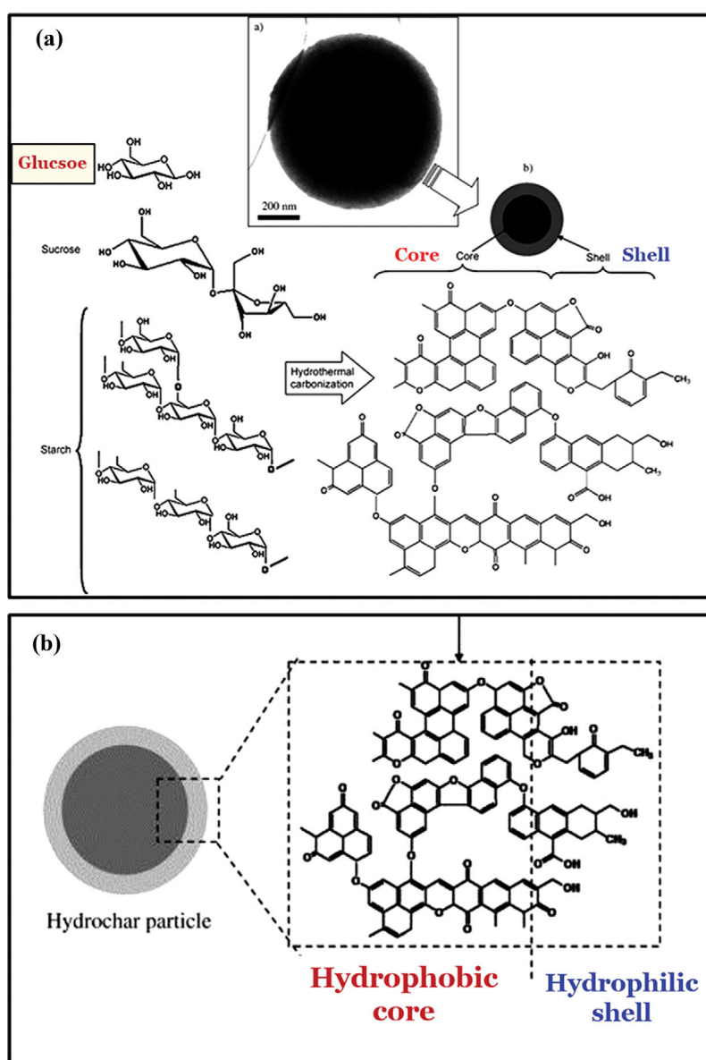
Fig. S1. (a) Mechanism of formation of spherical hydrochar particles from pure carbohydrate sources by hydrothermal carbonization; and (b) core-shell structure of spherical hydrochar (adapted from Sevilla and Fuertes [1]).
