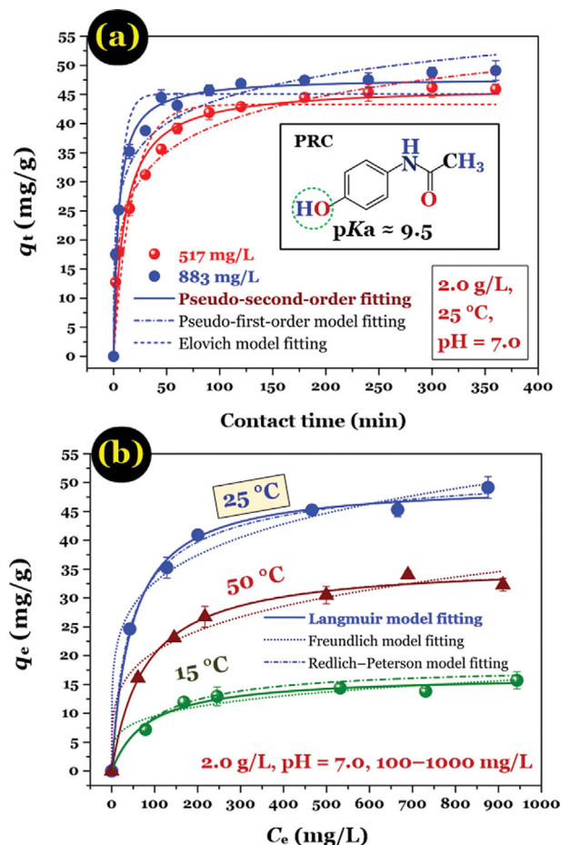
Fig. 7. (a) Adsorption kinetics and (b) isotherm of PRC onto the hematite-loaded spherical biochar (H-SB).
