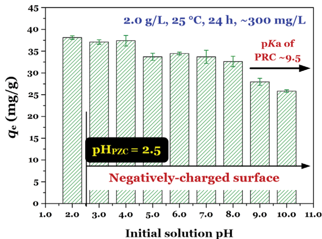
Fig. 6. Effect of solution pH on the adsorption capacity of the hematite-loaded spherical biochar (H-SB) towards PRC in solution.
