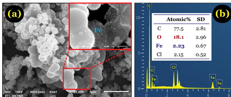
Fig. 1. (a) SEM and (b) EDS of the hematite-loaded spherical biochar (H-SB).
