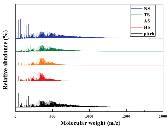
Fig. S1. MALDI-TOF spectra of pristine and molecular weight-controlled pitch.
