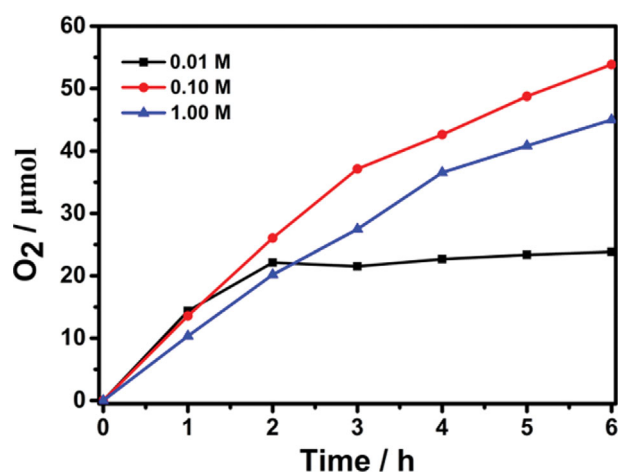
Fig. S1. Time courses of O 2 evolution in NaOH solution (10 mL) containing Na 2 S 2 O 8 (20 mM) and catalyst (5 mg) at room temperature.
