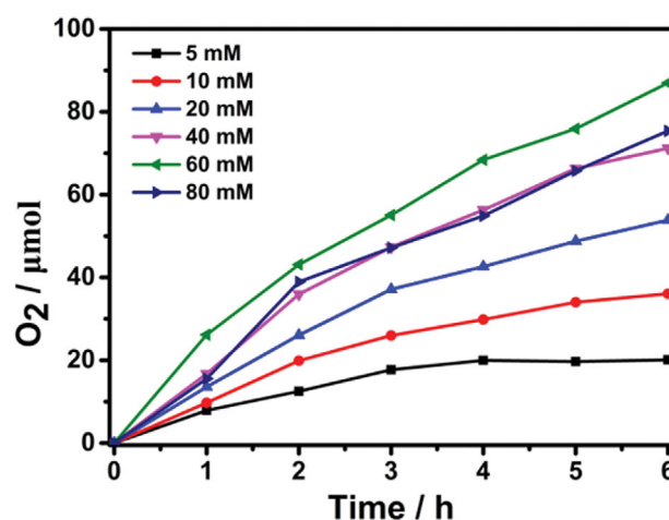
Fig. S2. Time courses of O 2 evolution in NaOH solution (0.10 M, 10 mL) containing catalyst (5 mg) at room temperature.
