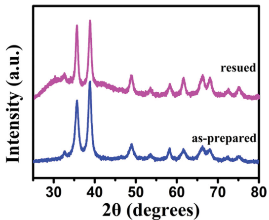
Fig. S5. XRD pattern of shuttle-like CuO-OH as-prepared and reused.
