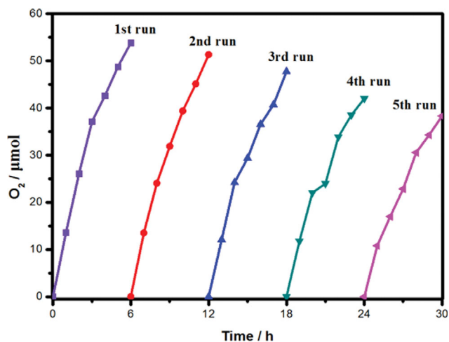
Fig. S4. The reuse of catalyst in WOR (reaction condition: NaOH solution: 0.10 M, 10 mL; Na 2 S 2 O 8 : 20 mM; catalyst: 5 mg; RT).
