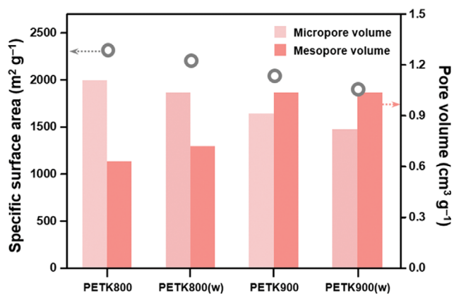
Fig. S3. Specific surface area and pore volumes of PETK800(w) and PETK900(w).
