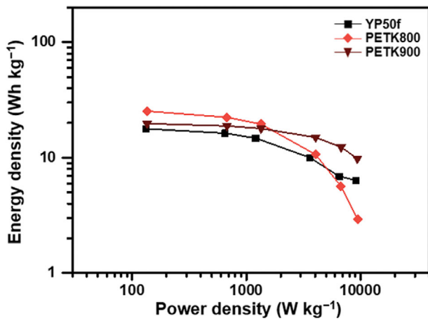
Fig. S1. Ragone plots of YP50f, PETK800, and PETK900.
