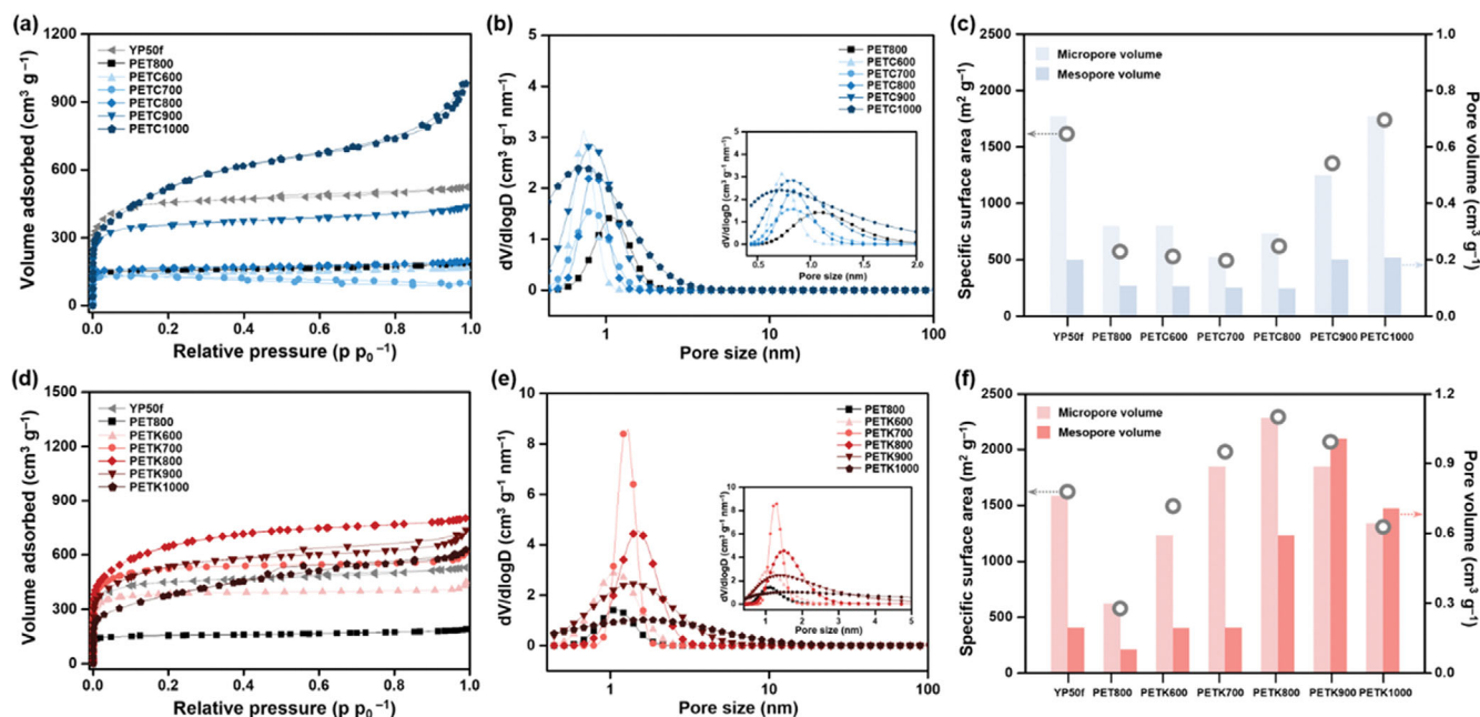
Fig. 2. (a) N_2 adsorption-desorption isotherms of PETCs, (b) pore size distributions of PETCs, (c) pore volumes of PETCs, (d) N_2 adsorption-desorption isotherm of PETKs, (e) pore size distributions of PETKs, and (f) pore volumes of PETKs.
