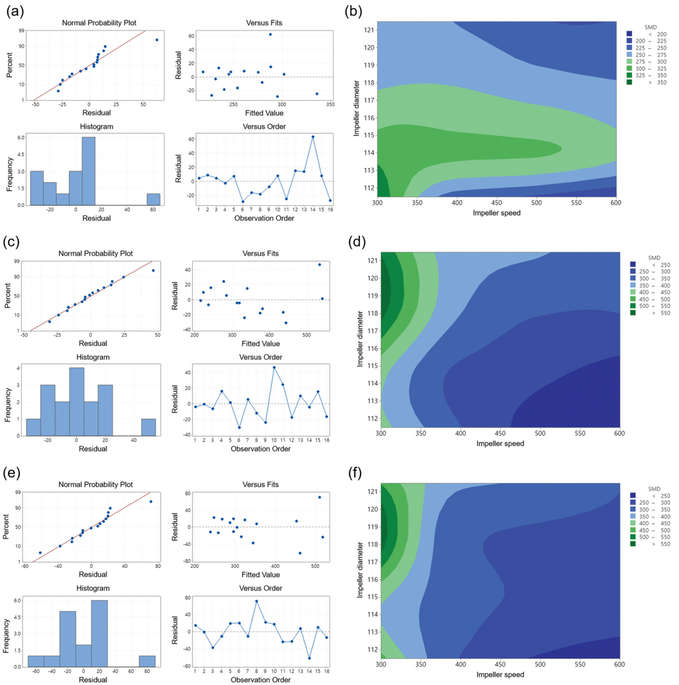
Fig. S4. DOE analysis for upper pitched paddle impeller diameter and impeller speed on Sauter mean diameter; (a) residual plots at port 1; (b) contour plot at port 1; (c) residual plots at port 2; (d) contour plot at port 2; (e) residual plots at port 3; (f) contour plot at port 3.
