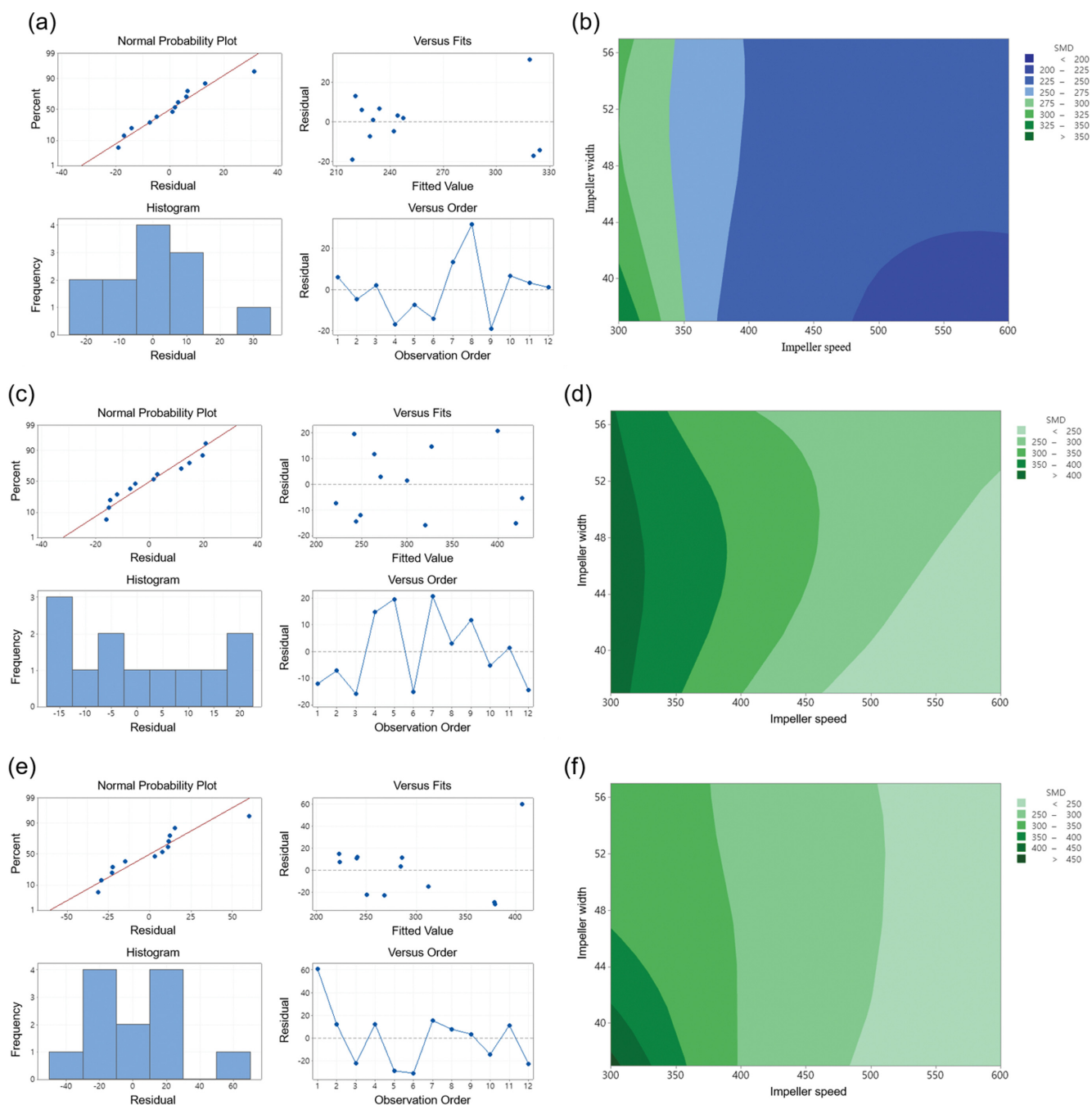
Fig. S5. DOE analysis for upper pitched paddle impeller width and impeller speed on Sauter mean diameter; (a) residual plots at port 1; (b) contour plot at port 1; (c) residual plots at port 2; (d) contour plot at port 2; (e) residual plots at port 3; (f) contour plot at port 3.
