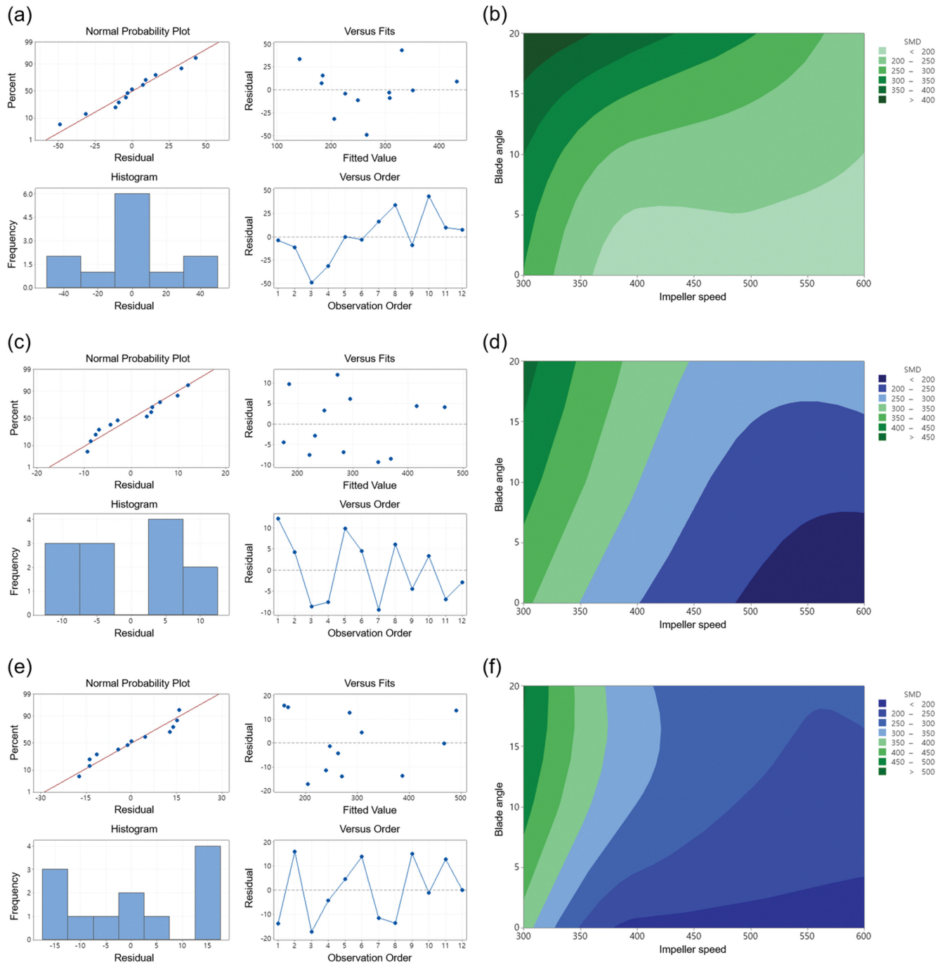
Fig. S3. DOE analysis for impeller blade angle and impeller speed on Sauter mean diameter; (a) residual plots at port 1; (b) contour plot at port 1; (c) residual plots at port 2; (d) contour plot at port 2; (e) residual plots at port 3; (f) contour plot at port 3.
