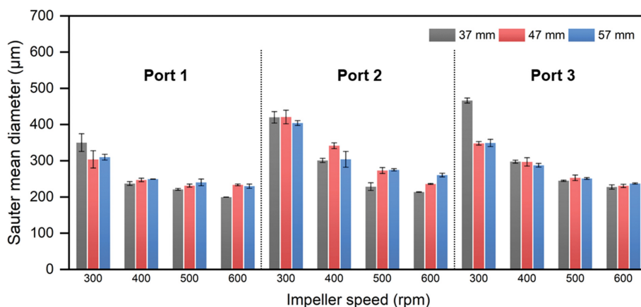
Fig. 12. Measured Sauter mean diameter with different impeller speed and upper 10° pitched paddle impeller blade width.
