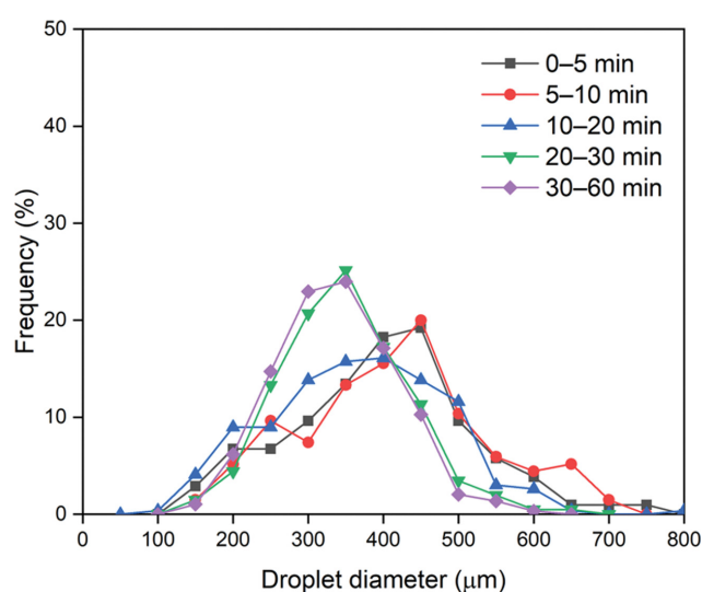
Fig. S1. Droplet size distributions for different time periods (at port 2, 300 rpm).
