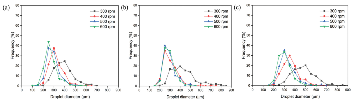
Fig. 8. Droplet size distribution at 10° pitched paddle-paddle impeller, port 1: (a) 114.5 mm diameter; (b) 118.5 mm diameter; (c) 121.5 mm diameter.
