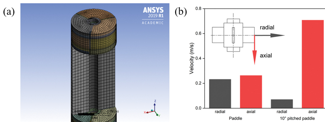
Fig. S2. CFD layout for the stirred liquid-liquid reactor with a dual impeller system; (a) mesh for the impeller zone and the impeller shaft; (b) average axial and radial velocities calculated by CFD study at the upper impeller of the paddle-paddle and 10° pitched paddle-paddle system.
