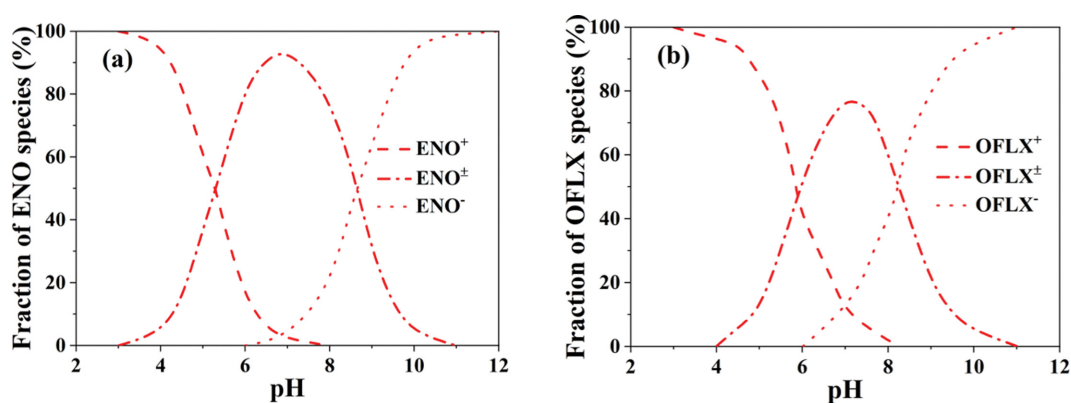
Fig. S4. Species of ENO (a) and OFLX (b) at different pH.
