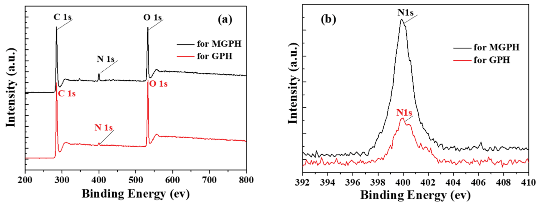
Fig. S2. XPS survey (a) and N1s XPS spectrum (b) of MGPH and GP.
