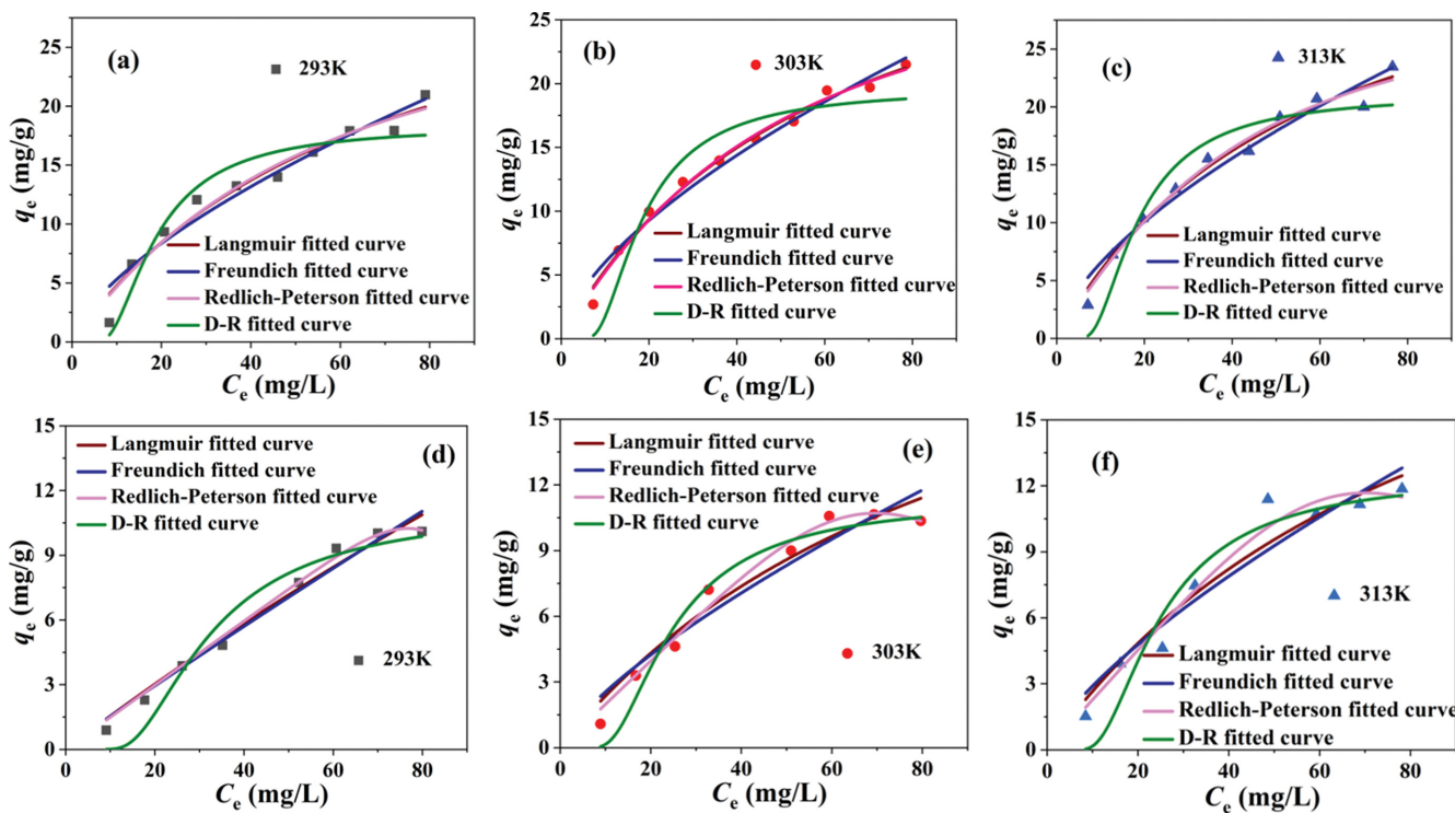
Fig. S5. The non-linear fitted curves with different equilibrium models for ENO (a), (b), (c) and OFLX (d), (e), (f) at 293 K, 303 K and 313 K, respectively.
