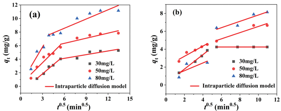
Fig. S7. The intraparticle diffusion plot for adsorption of ENO (a) and OFLX (b) at different concentrations.
