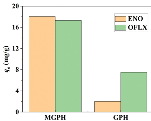
Fig. S8. The comparison of ENO and OFLX adsorption capacity onto MGPH and GPH.
