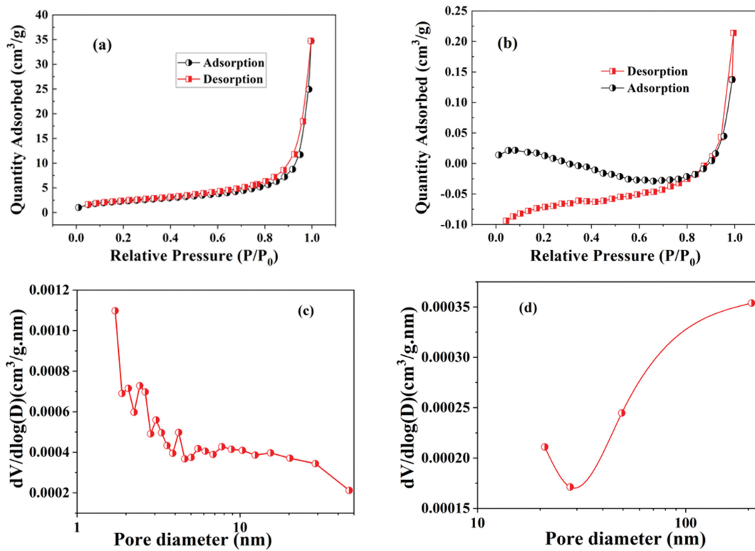
Fig. S1. N 2 adsorption-desorption isotherm (a), (b) and pore distribution (c), (d) of MGPH (a), (c) and GP (b), (d).
