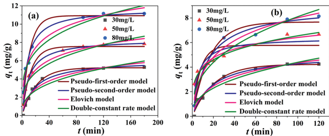
Fig. S6. Effect of contact time and initial concentration for ENO (a) and OFLX (b) adsorption onto MGPH.
