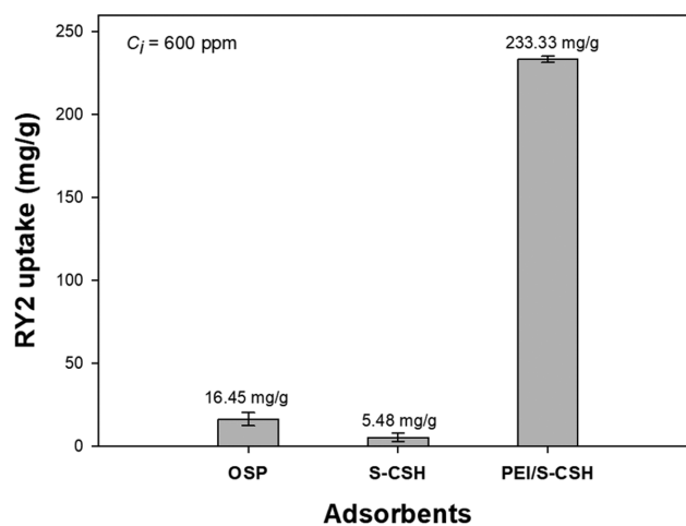
Fig. S2. Adsorption of RY2 onto different samples (OSP, S-CSH, and PEI/S-CSH). (Experimental conditions: pH 2; volume of solution, 30 mL; mass of adsorbent, 30 mg; initial RY2 concentration, 600 mg/L).
