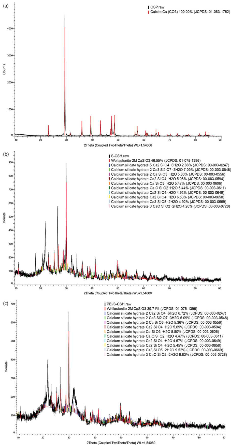
Fig. S3. X-ray diffraction patterns of (a) OSP, (b) S-CSH, and (c) PEI/S-CSH by using DIFFRAC.SUITE™ software.
