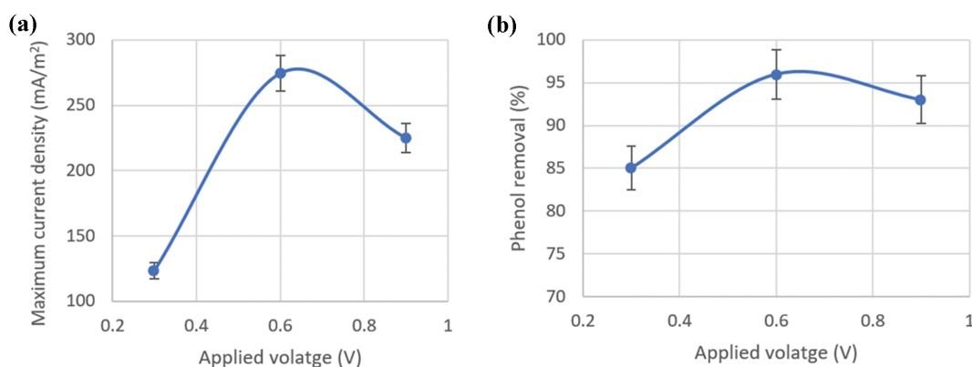
Fig. 3. The change of (a) maximum current density and (b) phenol removal under different applied voltages.
