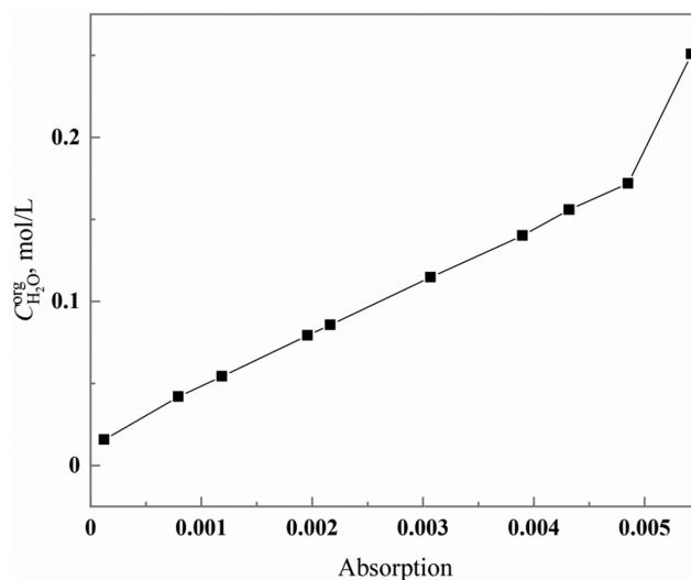
Fig. S5. Relationship between peak intensity and moisture content at 1,645\text{ cm}^{-1} .
