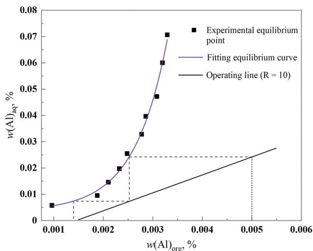
Fig. 16. Equilibrium isotherm for Al scrubbing at 80 °C. ( w(\text{P}_2\text{O}_5)_{\text{org}} = 15.03\% , w(\text{P}_2\text{O}_5)_{\text{scrubbing solution}} = 50.47\% ).
