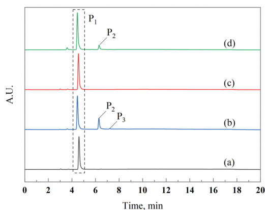
Fig. S2. Distribution of polyphosphoric acid in the extraction process by TBP. R_0=6 , Stirring rate=300 rpm (linear velocity=0.785 m/s), \phi_{\text{TBP}}=80\% , T=353.2\text{ K} , extraction time=30 min, centrifugal speed=3,000 rpm (5,205.4 g), centrifugal time=10 min. (a) The raffinate of the recycled extractant; (b) the raffinate of the "fresh" extractant; (c) the stripping acid of the recycled extractant; (d) the stripping acid of the "fresh" extractant.
