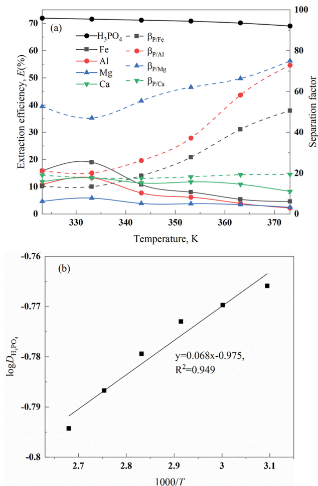
Fig. 8. (a) Effect of the temperature on the \text{H}_3\text{PO}_4 , Fe, Al, Mg and Ca extraction. R_0=6 , stirring rate= 300\text{ rpm} (linear velocity= 0.785\text{ m/s} ), \phi_{\text{TBP}}=80\% , T=353.2\text{ K} , extraction time= 30\text{ min} , centrifugal speed= 3,000\text{ rpm} ( 5,205.4\text{ g} ), centrifugal time= 10\text{ min} , extraction time= 30\text{ min} . (b) Linear fitting of \log D_{\text{H}_3\text{PO}_4} to 1,000/T .
