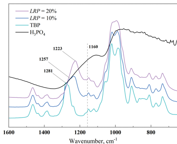
Fig. S7. The spectra of \text{H}_3\text{PO}_4 and TBP loaded with different amounts of \text{H}_3\text{PO}_4 .
