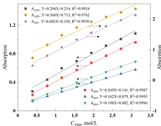
Fig. S3. Calibration curve for various concentrations of TBP solutions.
