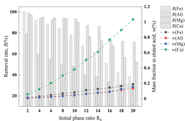
Fig. 15. Removal rate of metal ions by scrubbing under different R_0 conditions. Stirring rate=300 rpm (linear velocity=0.785 m/s), \varphi_{\text{TBP}}=80\% , w(\text{P}_2\text{O}_5)_{\text{scrubbing solution}}=50.47\% , w(\text{P}_2\text{O}_5)_{\text{org}}=15.03\% , w(\text{Fe})_{\text{org}}=0.007\% , w(\text{Al})_{\text{org}}=0.005\% , w(\text{Mg})_{\text{org}}=0.002\% , w(\text{Ca})_{\text{org}}=0.028\% , T=80^\circ\text{C} , and scrubbing time=10 min.
