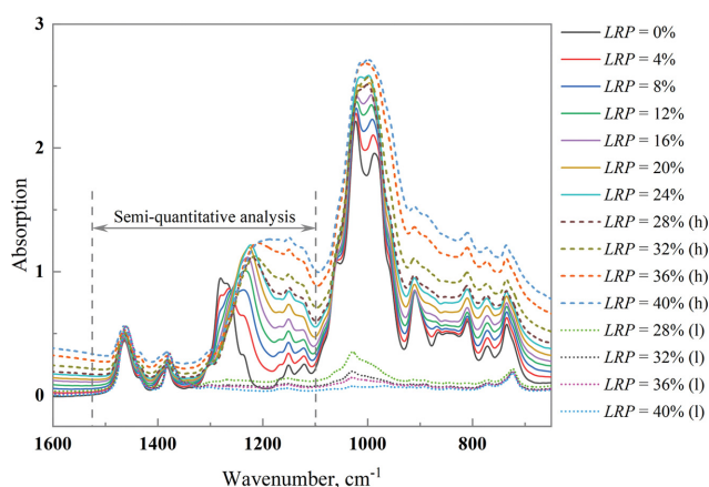
Fig. 12. The infrared spectra of the extractant loaded with different amounts of \text{H}_3\text{PO}_4 ("h" is for heavy phase, "l" is for light phase).
