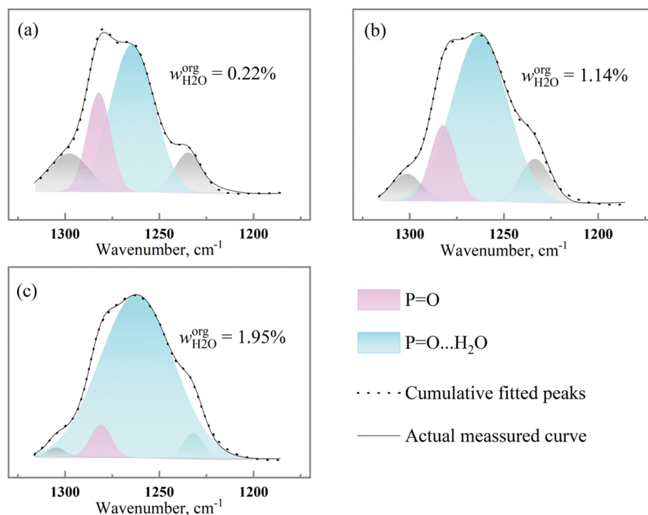
Fig. S6. The fitting results of TBP spectra for water contents of 0.22%, 1.14% and 1.95% at 1,320-1,180 \text{cm}^{-1} .
