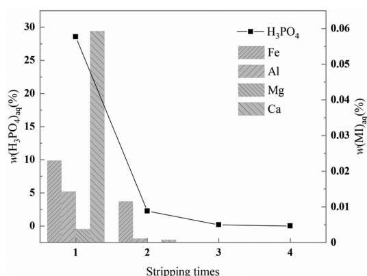
Fig. S1. Stripping acid composition at different stripping times. Initial phase ratio R_0=2 , stirring rate=300 rpm, temperature T=80^\circ\text{C} .
