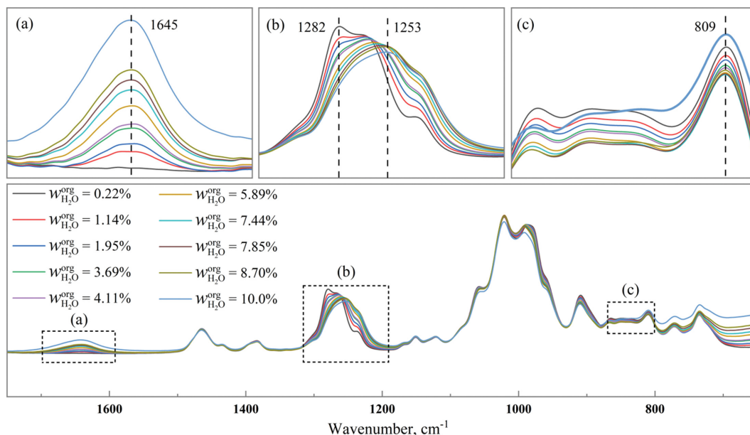
Fig. S4. Infrared spectra of TBP at different moisture contents.
