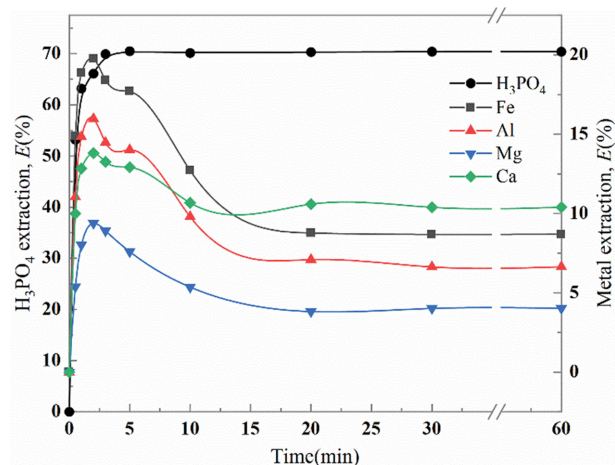
Fig. 3. Effect of the extraction time on the \text{H}_3\text{PO}_4 , Fe, Al, Mg, and Ca extraction rate. R_0=6 , stirring rate=300 rpm (linear velocity=0.785 m/s), \phi_{\text{TBP}}=80\% , T=80^\circ\text{C} , centrifugal speed=3,000 rpm (5,205.4 g), centrifugal time=10 min.
