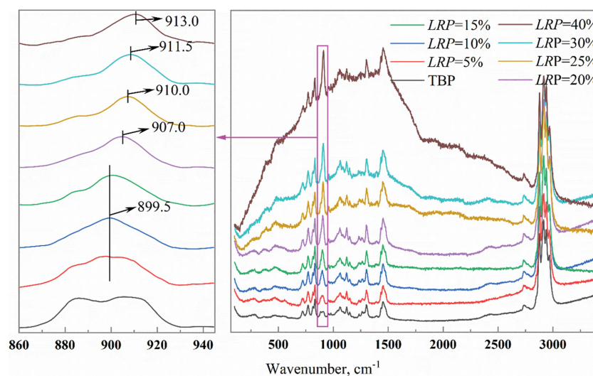
Fig. 14. Raman spectra at different LRP values.
