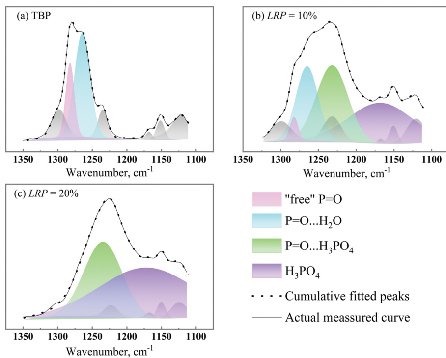
Fig. S8. The fitting results of TBP, LRP=10% and LRP=20% spectra at 1,350-1,180 \text{cm}^{-1} .
