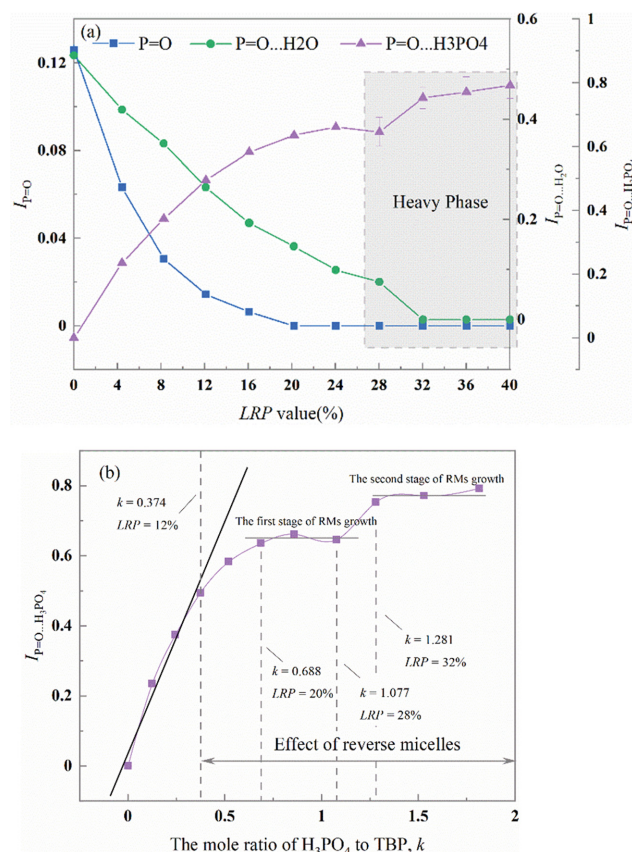
Fig. 13. (a) The I_{\text{P=O}} , I_{\text{P=O} \cdots \text{H}_2\text{O}} and I_{\text{P=O} \cdots \text{H}_3\text{PO}_4} versus LRP value. (b) The I_{\text{P=O} \cdots \text{H}_3\text{PO}_4} versus the mole ratio k of \text{H}_3\text{PO}_4 to TBP.
