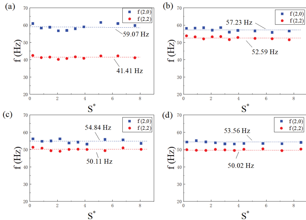
Fig. 11. Effects of the frequency of symmetrical shape oscillation as a function of dimensionless initial wall distance S^* at various surfactant concentrations: (a) pure water, (b) 100 ppm, (c) 400 ppm, and (d) 800 ppm; dashed line: mean frequency.
