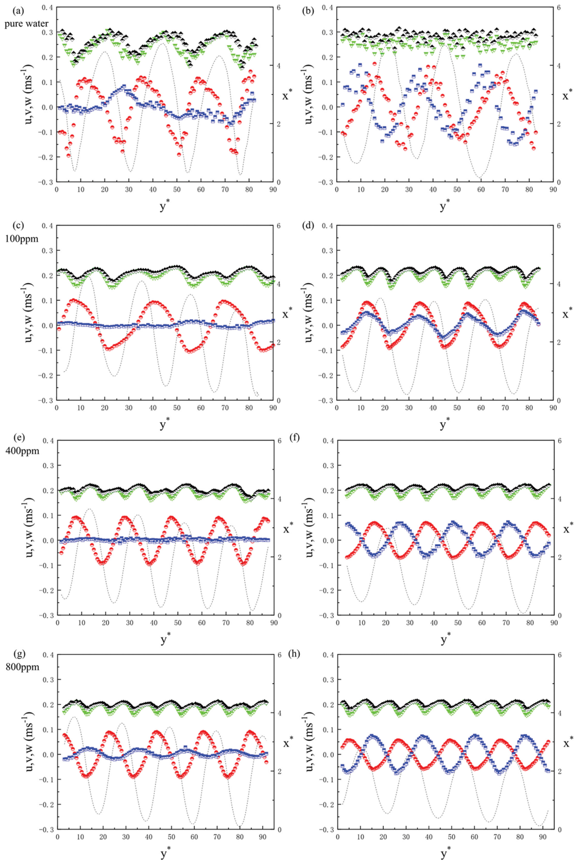
Fig. 7. Effect of various surfactant concentrations on the instantaneous velocity of collision at S^* \approx 0.22 and the instantaneous velocity of free-rising bubble ( x^* = x/req , y^* = y/req ): (a) (c) (e) (g): collision, (b) (d) (f) (h): free-rising case; black: instantaneous velocity ( U ), green: vertical velocity ( v ), red: wall-normal velocity ( u ), blue: spanwise velocity ( w ), dotted line: the trajectory of bubbles.
