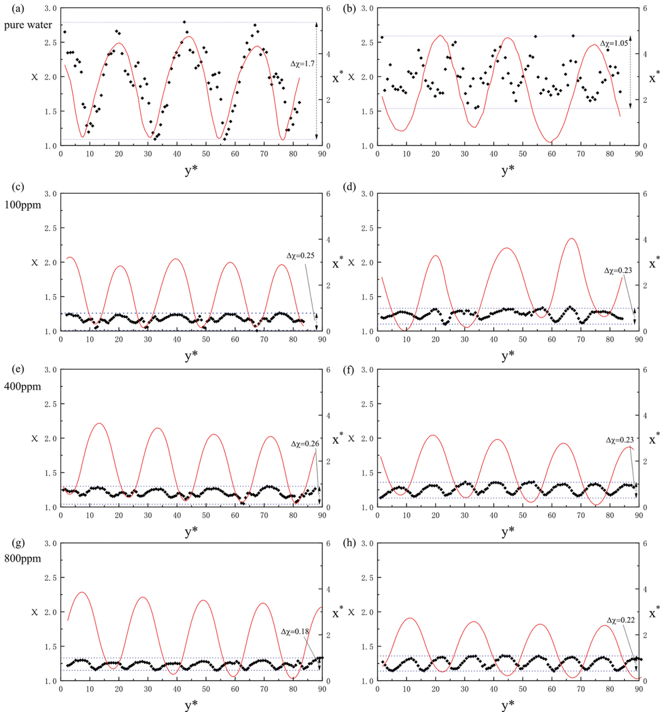
Fig. 9. Effect of various surfactant concentrations on the aspect ratio of collision at S^* \approx 0.22 and the free-rising case in the x - y plane: (a) (c) (e) (g): collision at S^* \approx 0.22 , (b) (d) (f) (h): free-rising case; black point: the aspect ratio of the bubble, red line: the trajectory of the bubble.
