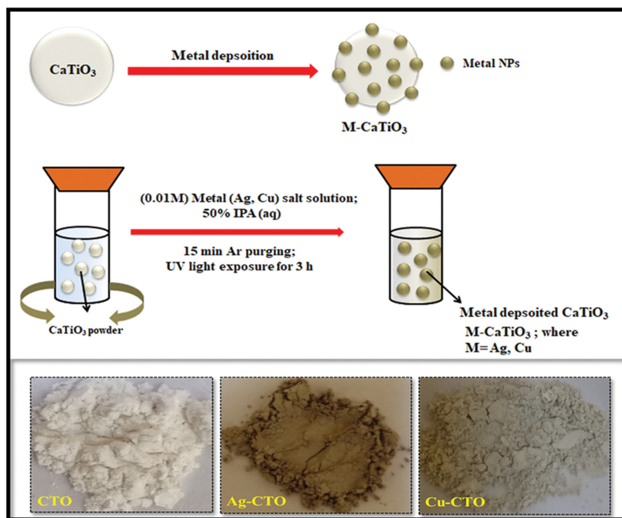
Scheme 2. Experimental procedure for photodeposition of M (M=Ag, Cu) NPs onto CaTiO 3 .
