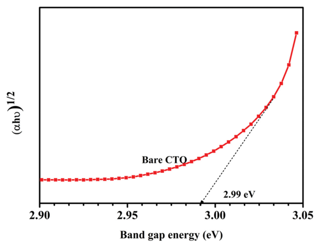
Fig. S1. (a) UV-DRS Tauc plot of bare \text{CaTiO}_3 (CTO).
