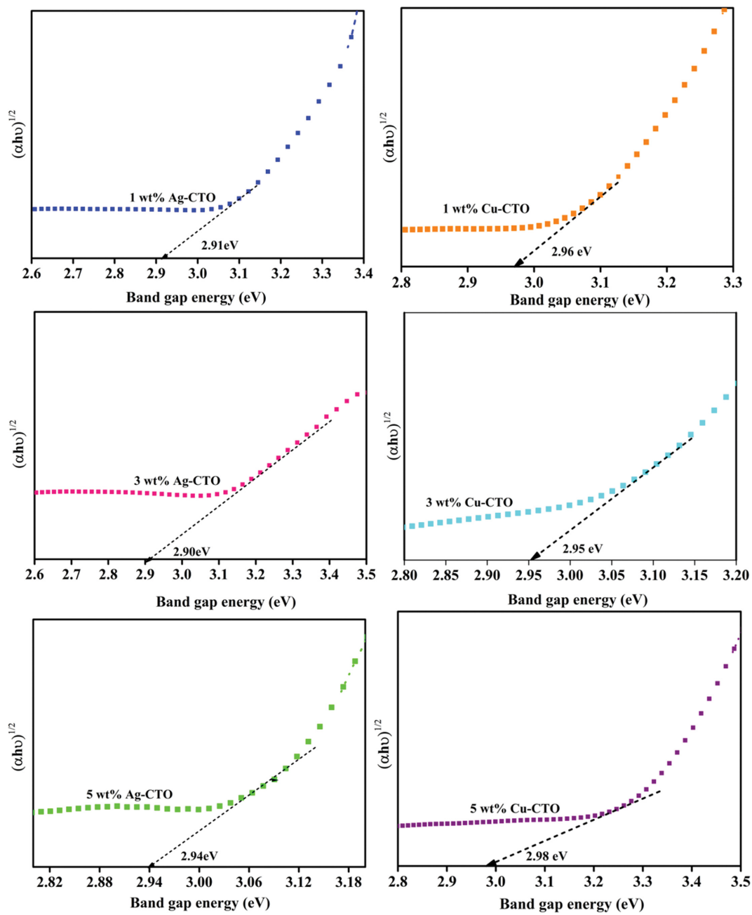
Fig. S1. (b) UV-DRS Tauc plot of various 1, 3, 5 wt% Ag/Cu-CTO samples.
