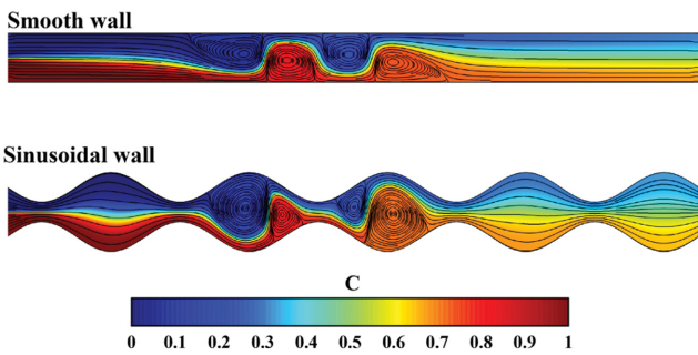
Fig. 13. Concentration distribution and streamlines in microchannels with straight and sinusoidal walls at \phi=0.03\% , d=1,000 \mu\text{m} , a=13.75 \text{ mm} , and \dot{Q}=25 \mu\text{l/min} .
