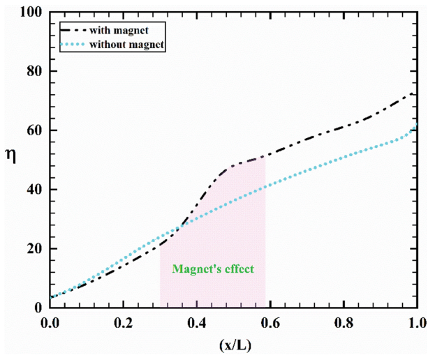
Fig. 5. Mixing index along the microchannel with and without the magnetic field at \varphi=0.03\% and \dot{Q}=25 \mu\text{l}/\text{min} .
