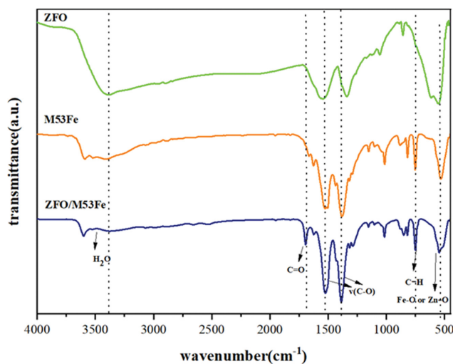
Fig. 4. FTIR spectra of different photocatalysts.
