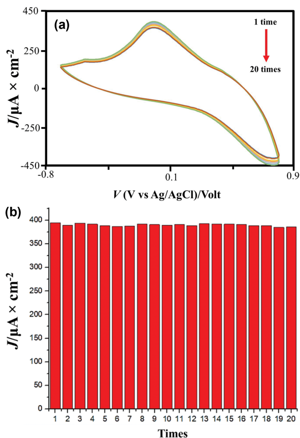
Fig. 12. Repeatability performance using TiO 2 -graphene nanocomposites: (a) Voltammogram repeatability analysis, (b) measurement of accuracy repeatability.
