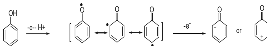
Fig. 1. Oxidation mechanism of phenol.
