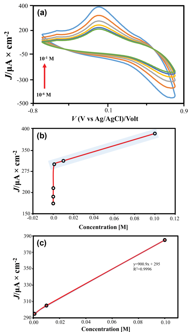
Fig. 9. Linearity and LoD of \text{TiO}_2 -graphene: (a) Phenol voltammogram at concentration of 10^{-6} M- 10^{-1} M, (b) Graph between phenol concentration and I_{pa} value, (c) Linearity area of phenol at concentration range of 10^{-3} M- 10^{-1} M.
