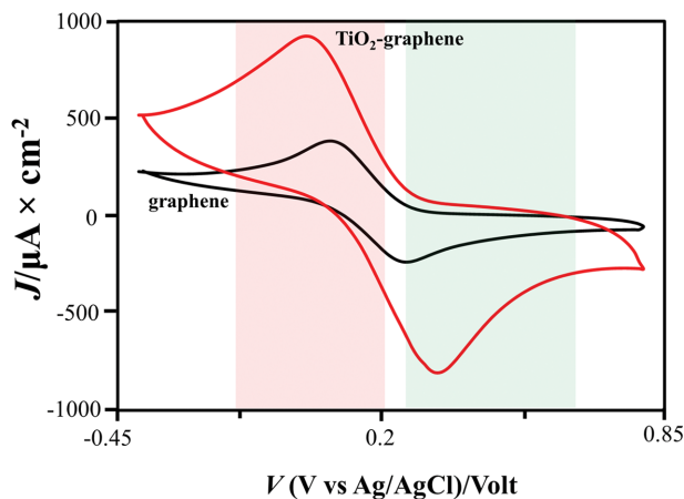
Fig. 8. Cyclic voltammogram of graphene nanosheet and \text{TiO}_2 -graphene in 0.1 M \text{K}_3[\text{Fe}(\text{CN})_6] .
