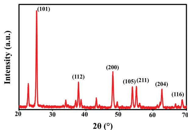
Fig. 3. XRD pattern of \text{TiO}_2 anatase by hydrothermal annealing.
