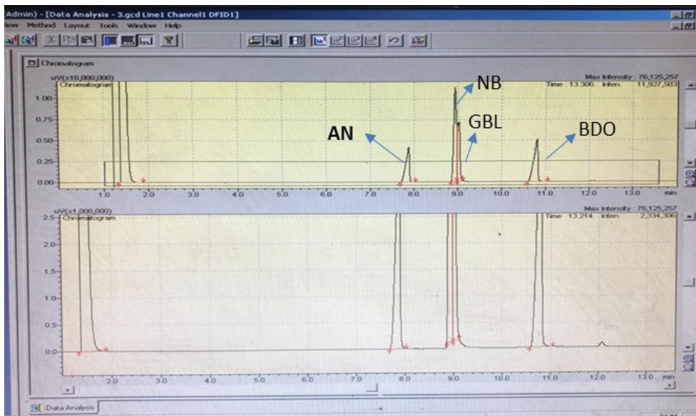
Fig. S3. GC-analysis of product mixture over 10CMA at 250 °C.
