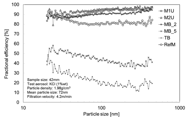
Fig. 5. Fractional collection efficiency vs. particle size for media and layers.
