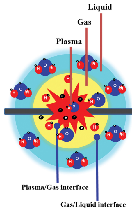
Fig. 3. The concept of liquid phase plasma process.
