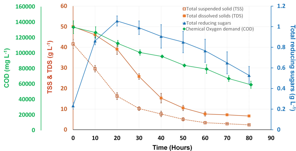
Fig. 3. The course of change in the physicochemical characteristics during the fermentation of vegetable waste biomass for the accumulation of organic acids [COD (Green), Total suspended solid (Brown-dotted line) Total dissolved solids (Brown-solid line) and Total reducing sugars (Blue)].
