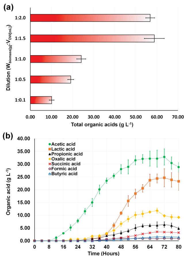
Fig. 2. Organic acids accumulation during acid fermentation by mixed cultures (a) Total organic acid accumulated in various dilutions of biomass with distilled water (W/V); (b) The course of accumulation of individual organic acids during fermentation under optimized conditions [Acetic acid (green), Lactic acid (orange), Oxalic acid (yellow), Propionic acid (black), Succinic acid (Red), Butyric acid (Blue) and Formic acid (brown)].
