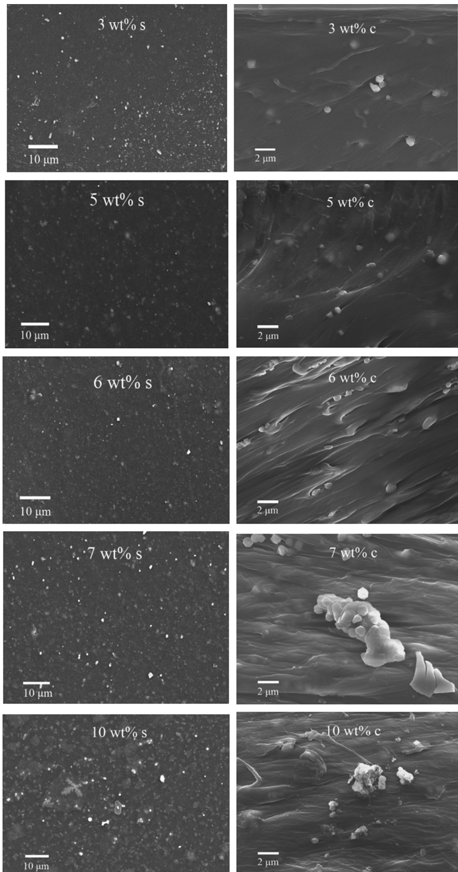
Fig. 4. SEM images of PEBA2533/NaY membranes containing different amounts of NaY grains (surface of the membranes is represented with s; cross-sections of the membranes are represented with c).
