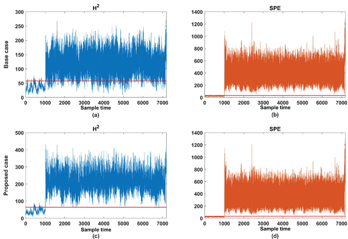
Fig. 12. Monitoring charts of fault 14 for the base case ((a) and (b)) and the proposed case ((c) and (d)).
