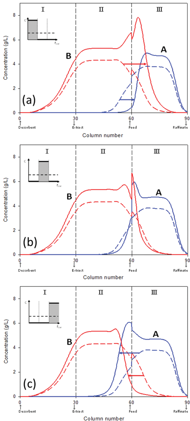
Concentrated feed at first third (a), middle third (b) and last third (c) of the switching time. The dashed line is concentration profile of three-zone SMB without ModiCon.
