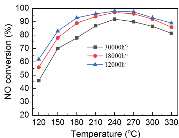
Fig. S3. Effect of gas hourly space velocity (GHSV) on NO conversion over Mn-Ce-Ti(N) catalyst.
