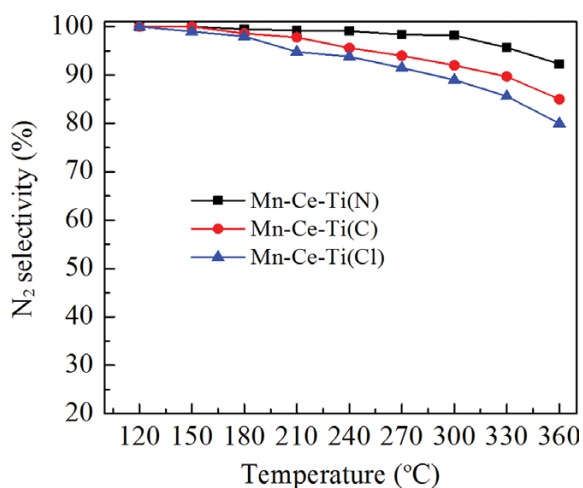
Fig. S1. N 2 selectivity over different Mn-Ce-Ti catalysts.
