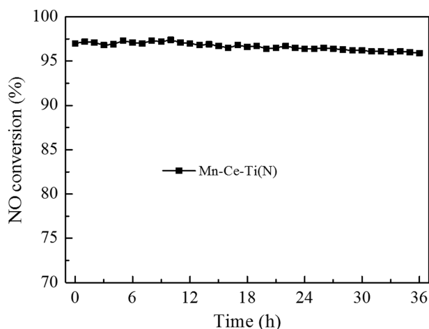
Fig. S2. Stability tests on the Mn-Ce-Ti(N) catalyst at 240 °C.
