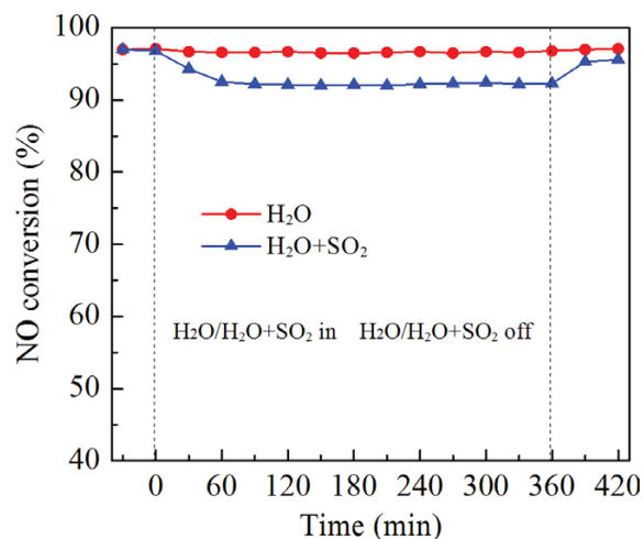
Fig. S4. Effect of H 2 O and SO 2 on the catalytic activity over Mn-Ce-Ti(N) catalyst at 240 °C. Reaction conditions: \varphi(\text{NO})=\varphi(\text{NH}_3)=500 ppm, \varphi(\text{H}_2\text{O})=5\% , \varphi(\text{SO}_2)=50 ppm, \varphi(\text{O}_2)=3\% , catalyst 5 mL, balance N 2 .
