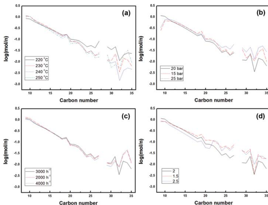
Fig. S2. Experimental Anderson-Schulz-Flory (ASF) distributions at various experimental cases such as reaction temperatures of 220-250 °C, reaction pressures of 15-25 bar, space velocities (SV) of 2,000-4,000 h -1 , and feed molar ratios of H 2 /CO=1.5-2.5.
