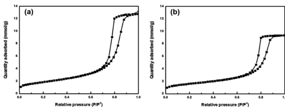
Fig. S1. N 2 adsorption-desorption isotherms of (a) \gamma -Al 2 O 3 itself (granule size of 1 mm), (b) fresh Co-Pt/Al 2 O 3 catalyst.
