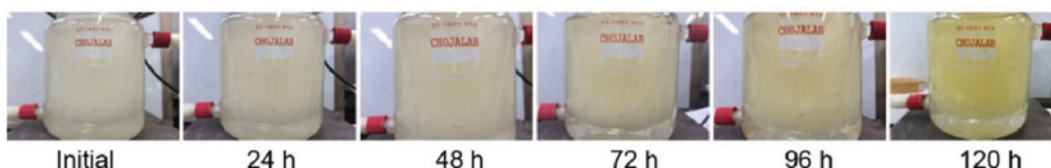
Fig. 5. Photographs of (a) aqueous glycine solution/oleic acid emulsion and (b) aqueous glycine solution/octanoic acid emulsion with aging time at 85 °C.
