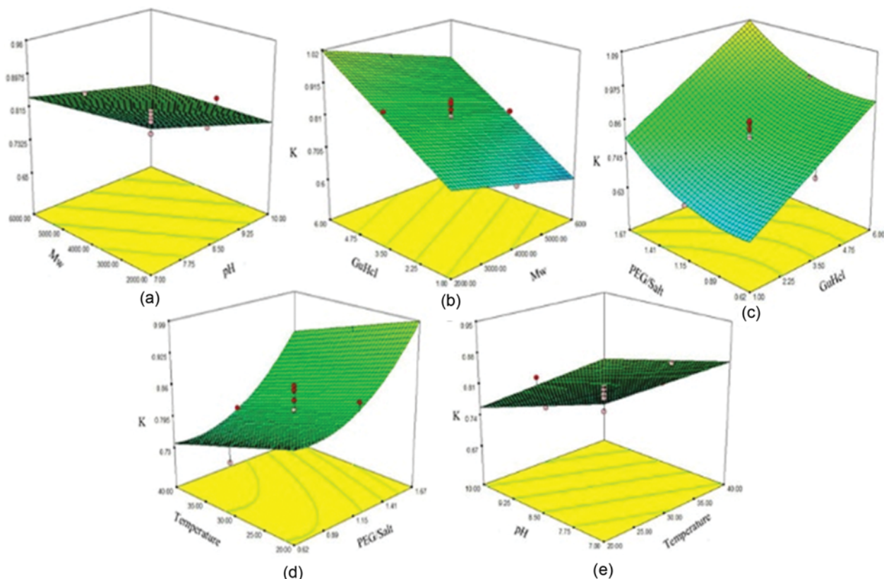
Fig. 7. Response surface plots for the effects of (a) molecular weight and initial solution pH; (b) GuHCl concentration and molecular weight; (c) GuHCl concentration and polymer/salt concentration; (d) polymer/salt concentration and temperature; (e) initial solution pH and temperature; circle is design point.
