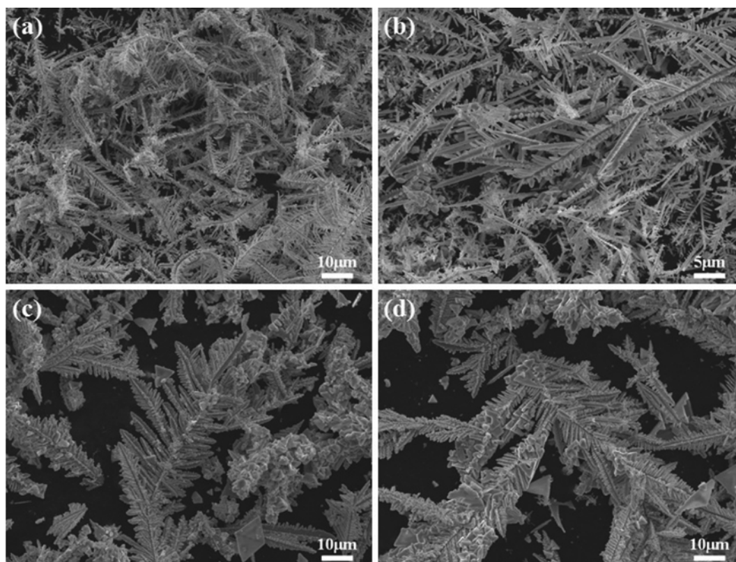
Fig. 3. FE-SEM images of dendritic copper powders obtained in electrolytes (a) 0.5 M \text{H}_2\text{SO}_4 , 0.1 M \text{CuSO}_4 and 0.1 M KCl, (b) 0.5 M \text{H}_2\text{SO}_4 , 0.1 M \text{CuSO}_4 and 0.1 M NaCl, (c) 0.5 M \text{H}_2\text{SO}_4 , 0.1 M \text{CuSO}_4 and 0.1 M KBr, and (d) 0.5 M \text{H}_2\text{SO}_4 , 0.1 M \text{CuSO}_4 and 0.1 M NaBr, respectively.
