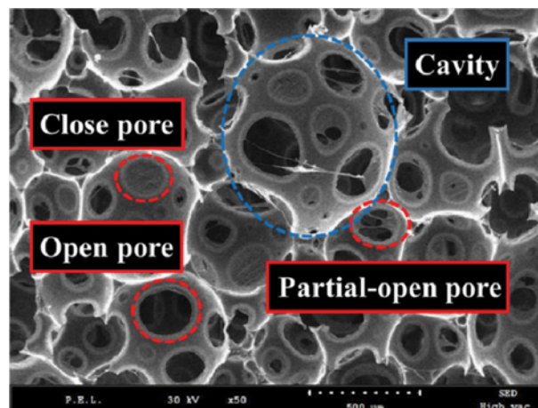
Fig. 2. SEM image defining areas for cavity and three types of pores (open, partial-open and close).
