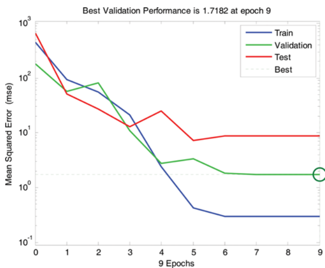
Fig. S3. Error and learning curve of the neural network.
