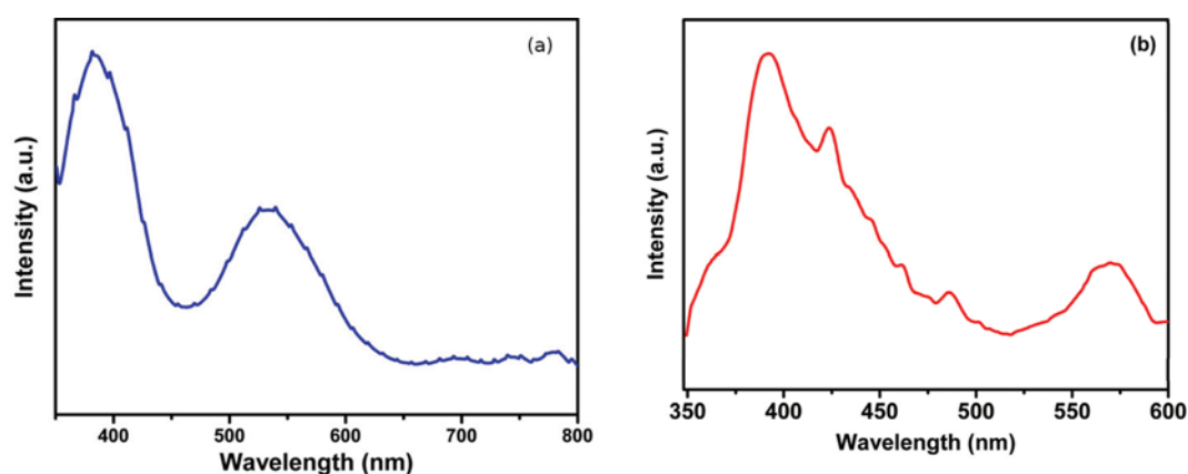
Fig. S4. PL spectra for pure ZnO (a) without milling and (b) with milling process.
