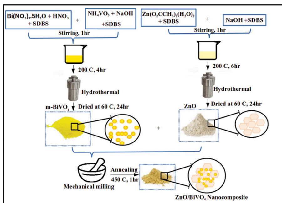
Fig. S1. Schematic showing preparation of ZnO-BiVO 4 nanocomposite.
