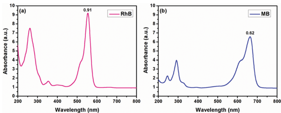
Fig. S3. UV-vis spectra for (a) RhB and (b) MB dye.
