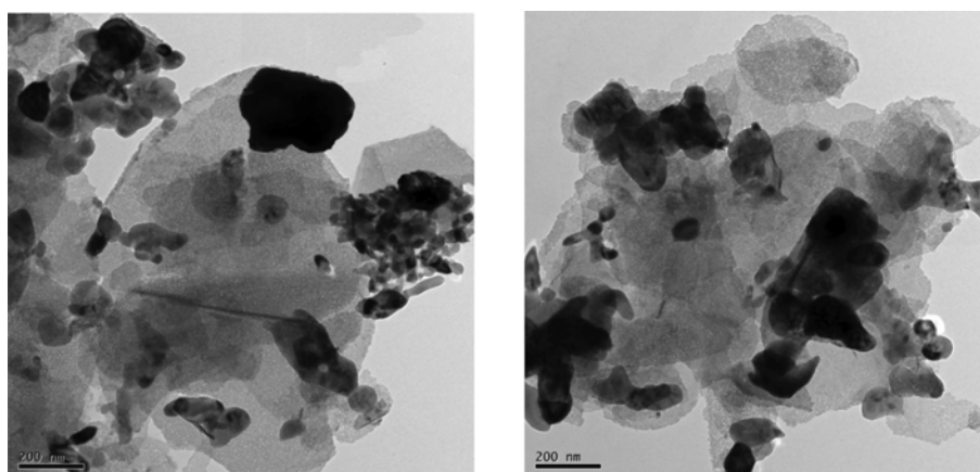
Fig. S2. TEM images of composite samples revealing complete attachment of BiVO 4 nanoparticles to ZnO nanosheets at lower magnification scale.
