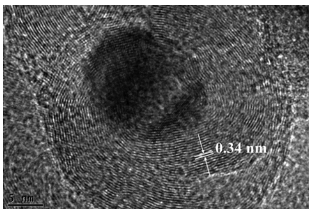
Fig. S1. The TEM image of the spent Ni-IM catalyst after 100 h stability test.
