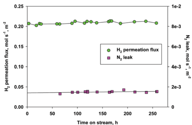
Fig. 6. Long-term stability of membrane KIER-Pd-201-20 at 773 K.
