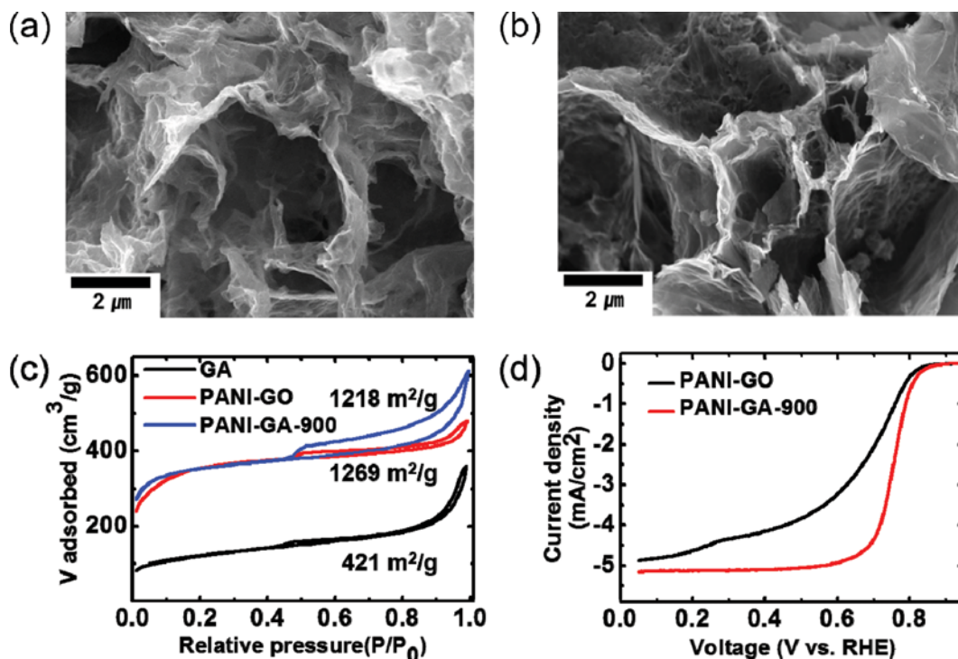
Fig. 1. SEM images of (a) GA and (b) PANI-GA-900. (c) Nitrogen adsorption-desorption isotherm curves for GA, PANI-GO and PANI-GA-900. (d) Linear sweep voltammetry results for PANI-GO and PANI-GA-900; the loading amount was 600 μg/cm 2 , the catalyst ink concentration was 10 mg/ml, the rotation speed of the electrode was 1,600 rpm, and the scan rate was 10 mV/s in O 2 -saturated 0.5 M H 2 SO 4 electrolyte.
