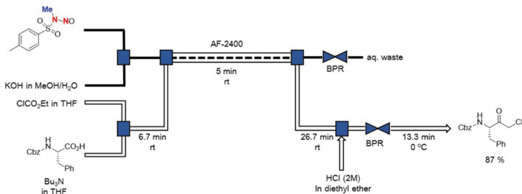
Fig. 3. Scheme of generation of an anhydrous and ethereal solution of diazomethane and formation of \alpha -diazo ketone in a continuous-flow tube-in-tube system. AF-2400 membrane with 100 \mu m thickness (0.8 mm i. d., 1 mm o.d., 4 m length) and PTFE outer (1.59 mm i.d., 3.2 mm o.d., 4 m length) tubing system. J. Org. Chem. , 79, 1555 (2014).
