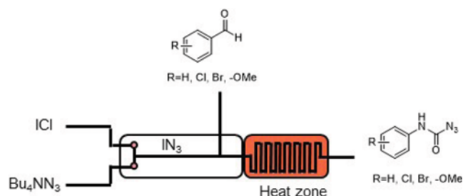
Fig. 18. In-situ generation of IN 3 and utilization for formation of carbonyl azide. After mixing, the aldehyde with the iodine azide reagent passes through a capillary (196- \mu L volume) at 80 °C (heat zone). Beilstein J. Org. Chem. , 5, 30 (2009).
