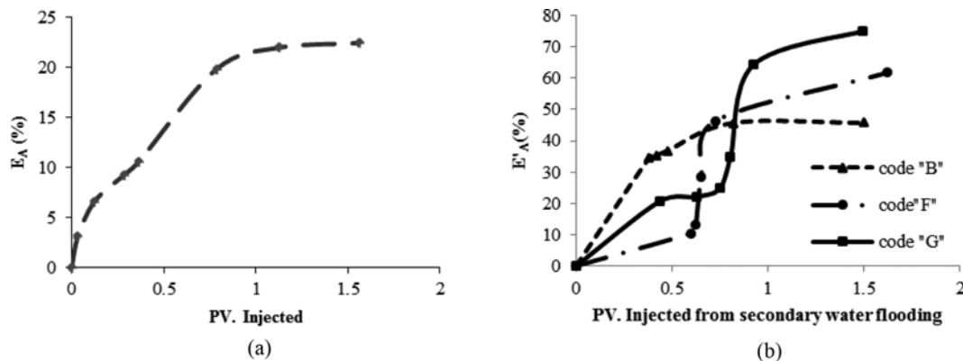
Fig. 9. Areal sweep efficiency of (a) primary water flooding, (b) secondary water flooding.
