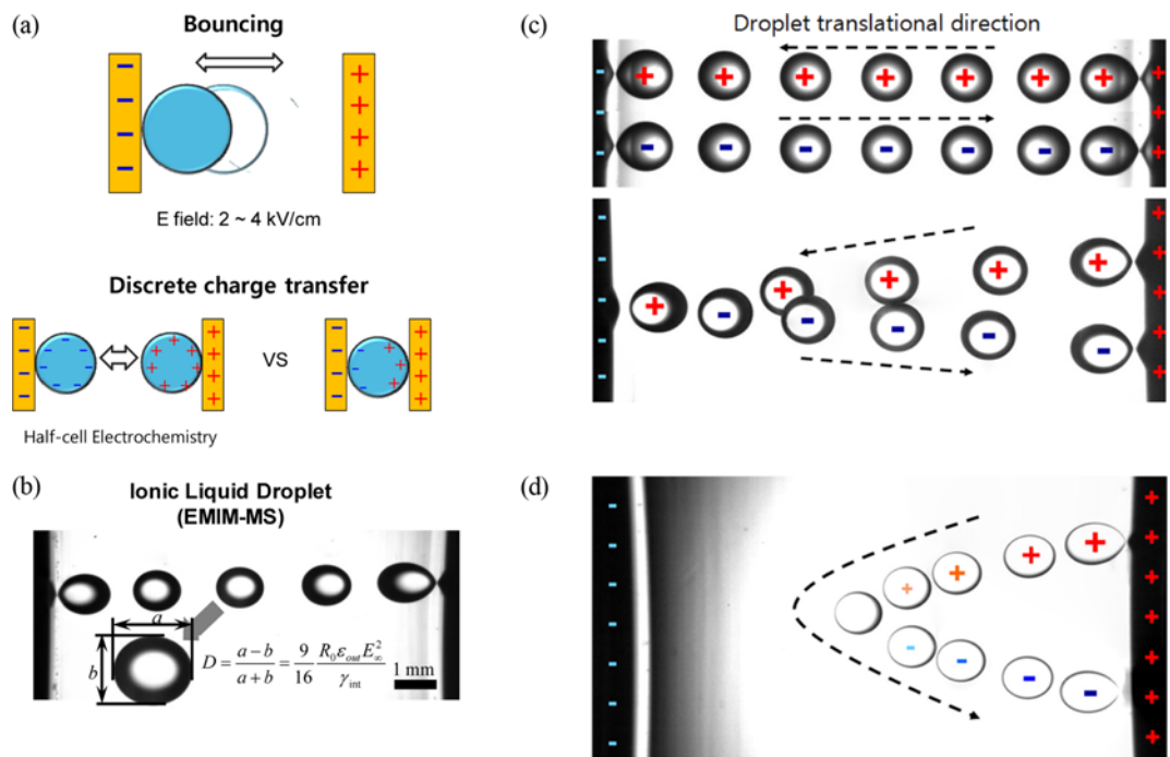
Fig. 5. (a) Discrete charge transfer by ECD. (b) Interfacial tension measurement by ECD. (c) ECD motion of a 300 nL water droplet (top) and a 400 nL BMIM-MS ionic liquid droplet (bottom). (d) Retreating behavior of a 400 nL EMIM-NTf2 ionic liquid droplet. Adapted from ref. [57-58]. Copyright 2013, 2014 American Chemical Society.
