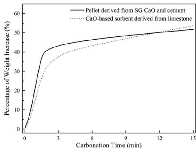
Fig. 3. Carbonation kinetics of the pellet and limestone during the first cycle.
