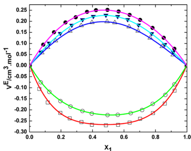
Fig. 1. Variation of excess molar volume ( V^E ) with mole fraction ( x_1 ) of N-ethylaniline in the binary liquid mixtures of N-ethylaniline with chlorobenzene (□), bromobenzene (○), 1,2-dichlorobenzene (△), 1,3-dichlorobenzene (▼) and 1,2,4-trichlorobenzene (●) at 303.15 K.
