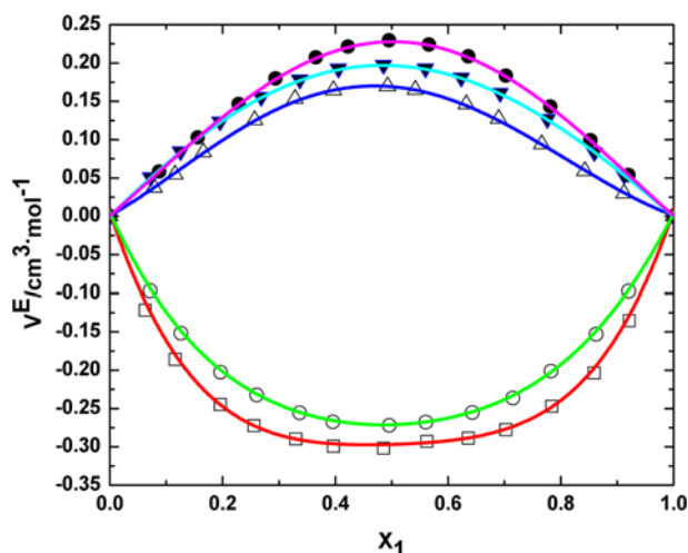
Fig. 2. Variation of excess molar volume ( V^E ) with mole fraction ( x_1 ) of N-ethylaniline in the binary liquid mixtures of N-ethylaniline with chlorobenzene (□), bromobenzene (○), 1,2-dichlorobenzene (△), 1,3-dichlorobenzene (▼) and 1,2,4-trichlorobenzene (●) at 308.15 K.
