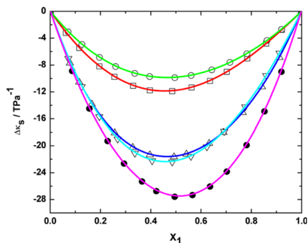
Fig. 3. Deviation in isentropic compressibility ( \Delta\kappa_s ) with mole fraction ( x_1 ) of N-ethylaniline in the binary liquid mixtures of N-ethylaniline with chlorobenzene (□), bromobenzene (○), 1,2-dichlorobenzene (△), 1,3-dichlorobenzene (▼) and 1,2,4-trichlorobenzene (●) at 303.15 K.
