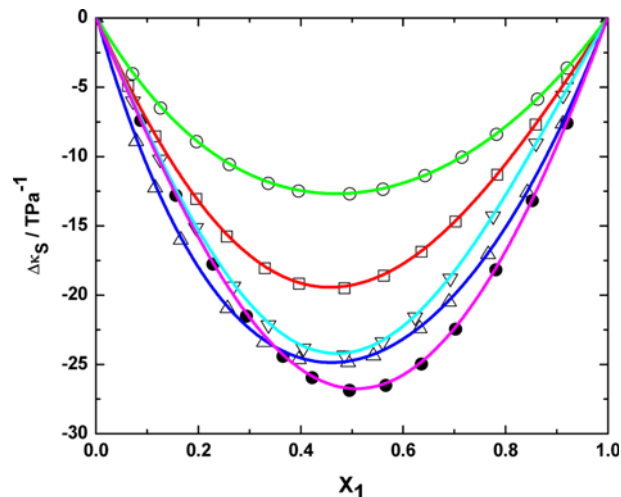
Fig. 4. Deviation in isentropic compressibility ( \Delta\kappa_s ) with mole fraction ( x_1 ) of N-ethylaniline in the binary liquid mixtures of N-ethylaniline with chlorobenzene (□), bromobenzene (○), 1,2-dichlorobenzene (△), 1,3-dichlorobenzene (▼) and 1,2,4-trichlorobenzene (●) at 308.15 K.
