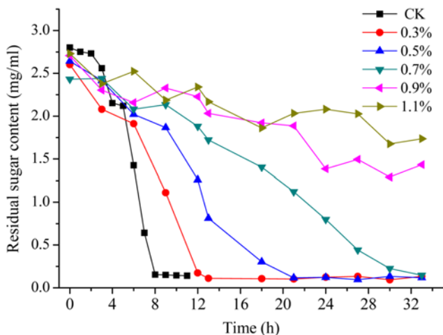
Fig. 3. Residual sugar curve of yeast in low concentration ionic liquid bmim[PF6].
