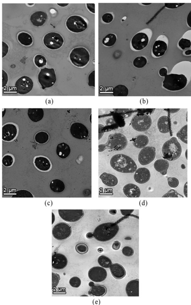
Fig. 9. Transmission electron microscope photos of yeast in different treated methods. (a) blank control; (b) 20% ionic liquid; (c) 40% ionic liquid; (d) 20% benzyl alcohol; (e) 14 MPa supercritical CO 2 .
