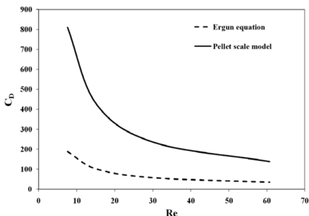
Fig. 10. Comparison of drag coefficient predicted by pellet scale model and Ergun equation ( e=0.4 ).
