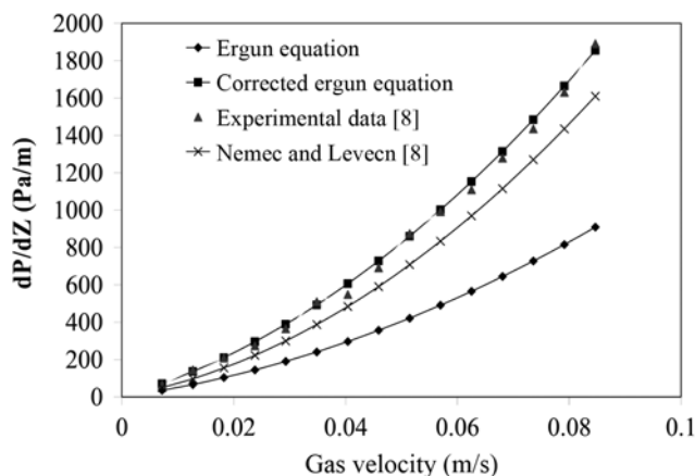
Fig. 13. Pressure drop prediction by Ergun equation, Nemeć and Levec model [8], corrected Ergun (This work) and experimental data [8], P=10 bars, L/d=5.35 , e=0.466 .
