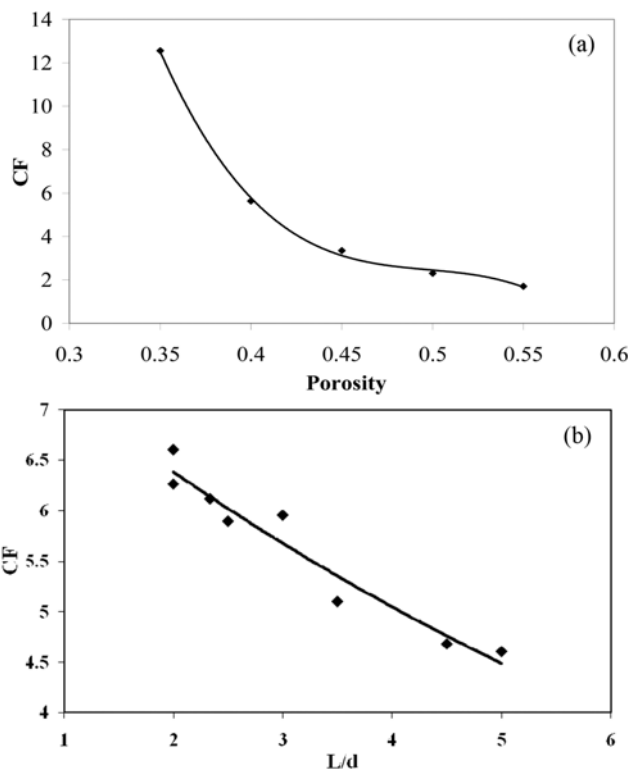
Fig. 11. Variations of correction factor (at constant Re=16.6 ) with (a) Porosity (b) Aspect ratio ( e=0.4 ).
