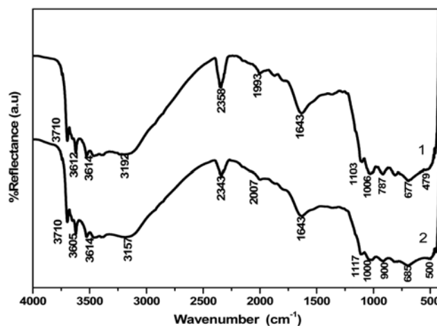
Fig. 7. FTIR spectra of iron ore slimes and Pb adsorbed sample (1. iron ore slime. 2. Iron ore slime sample adsorbed with lead ions).
