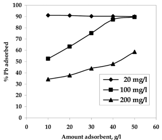
Fig. 9. Effect of amount of iron ore slimes on removal of lead ions. pH 5.1, agitation time 60 min, Temp: 300 K.
