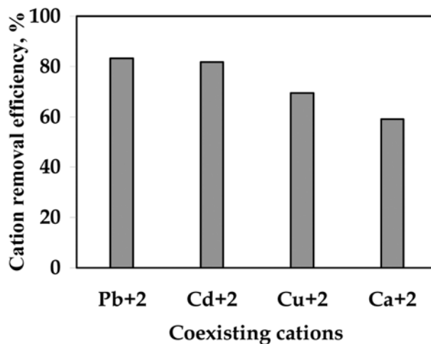
Fig. 15. Effect of coexisting cations on Pb(II) removal. Initial Pb(II) concentration 100 mg/l, adsorbent dose: 10 g/l, pH 5.1, T= 300 K.
