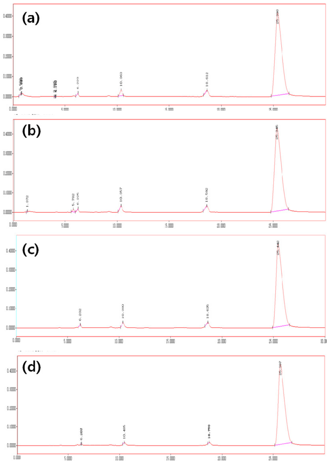
Fig. 6. HPLC data for the water layer after extraction of triphenyl phosphate (TPP) with a change of TBP added amount. (a) 10 g, (b) 20 g, (c) 30 g and (d) 40 g.
