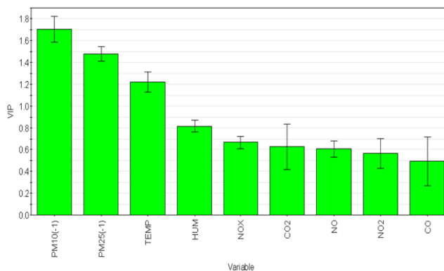
Fig. 7. PLS results as VIP plot.
