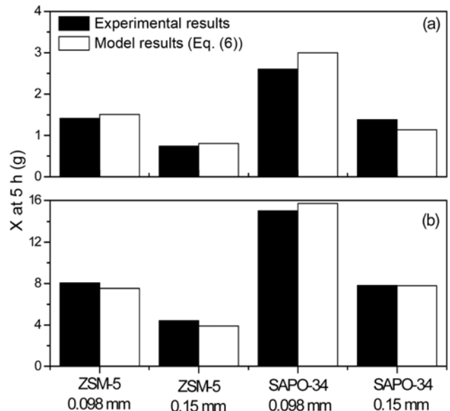
Fig. 6. Comparison of Zeeshan formulation and experimental results over a wide range (a) co-fluidized with ZSM-5 particles of density 1.68 \text{ g/cm}^3 and 2.7 \text{ mm} size, (b) co-fluidized with high density ceramic balls 2.64 \text{ g/cm}^3 and 0.7 \text{ mm} size.
