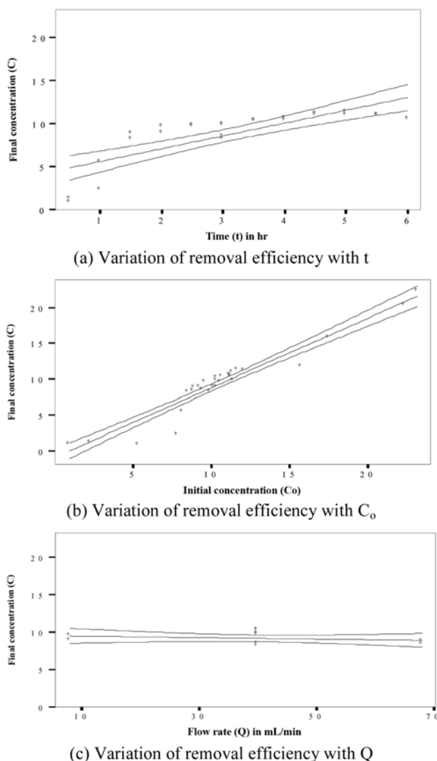
Fig. 9. Linear two-dimensional regression models.
