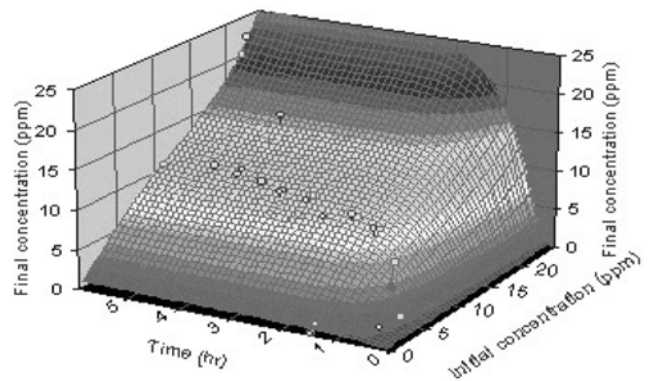
Fig. 12. Variation of final concentration of arsenic with C_0 and t .
