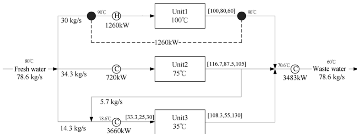
Fig. 16. The optimal network structure in example 2 (simultaneous).
