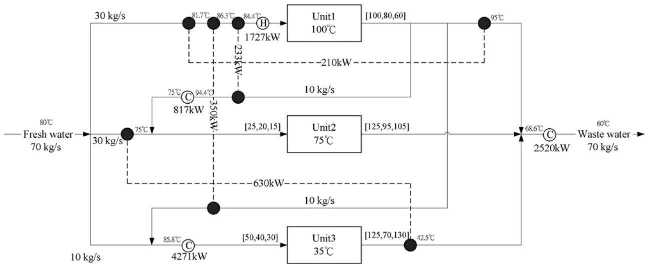
Fig. 15 The optimal network structure in example 2 (sequential).
